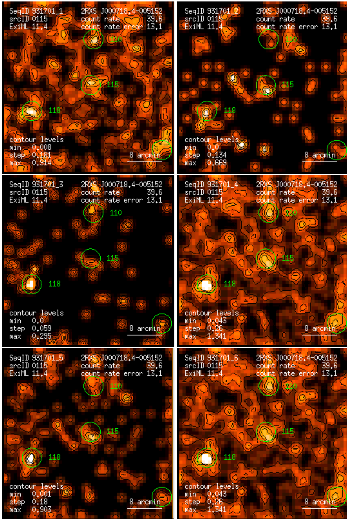
Figure 115: RASS 931701: detection 0115: band rate images, Gaussian filter: (1) PSPC channels 11 – 41, (2) 52 – 90, (3) 91 – 201, (4) 11 – 235, (5) 52 – 201, (6) 11 – 201. Broad band rates in counts/ks. Band rate contour levels in counts/ks/arcmin 2 .
