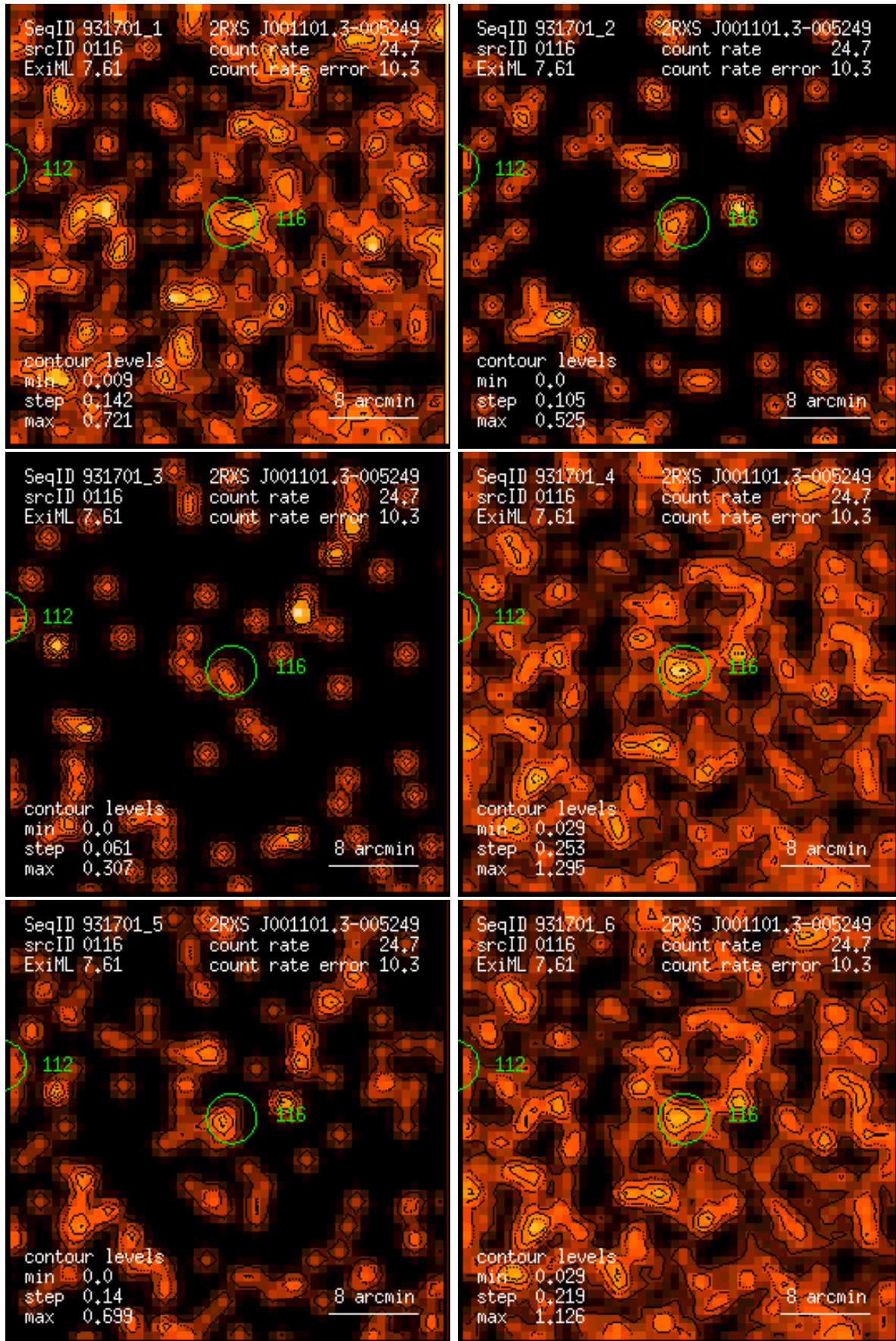
Figure 116: RASS 931701: detection 0116: band rate images, Gaussian filter: (1) PSPC channels 11 – 41, (2) 52 – 90, (3) 91 – 201, (4) 11 – 235, (5) 52 – 201, (6) 11 – 201. Broad band rates in counts/ks. Band rate contour levels in counts/ks/arcmin 2 .
