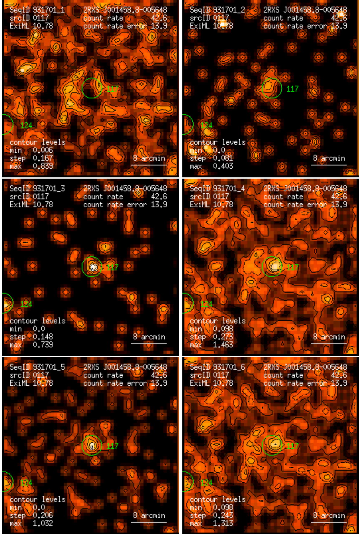
Figure 117: RASS 931701: detection 0117: band rate images, Gaussian filter: (1) PSPC channels 11 – 41, (2) 52 – 90, (3) 91 – 201, (4) 11 – 235, (5) 52 – 201, (6) 11 – 201. Broad band rates in counts/ks. Band rate contour levels in counts/ks/arcmin 2 .
