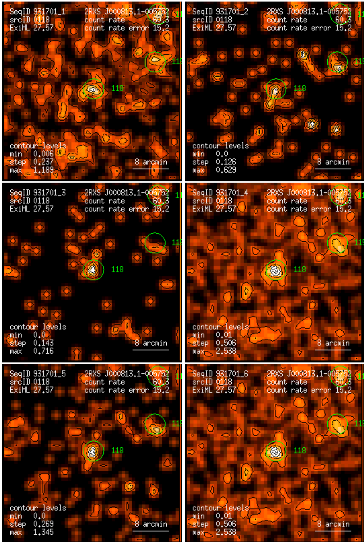
Figure 118: RASS 931701: detection 0118: band rate images, Gaussian filter: (1) PSPC channels 11 – 41, (2) 52 – 90, (3) 91 – 201, (4) 11 – 235, (5) 52 – 201, (6) 11 – 201. Broad band rates in counts/ks. Band rate contour levels in counts/ks/arcmin 2 .
