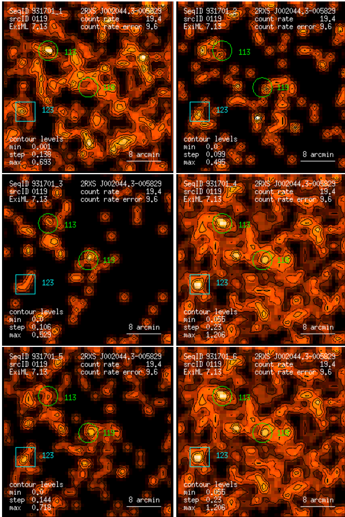
Figure 119: RASS 931701: detection 0119: band rate images, Gaussian filter: (1) PSPC channels 11 – 41, (2) 52 – 90, (3) 91 – 201, (4) 11 – 235, (5) 52 – 201, (6) 11 – 201. Broad band rates in counts/ks. Band rate contour levels in counts/ks/arcmin 2 .
