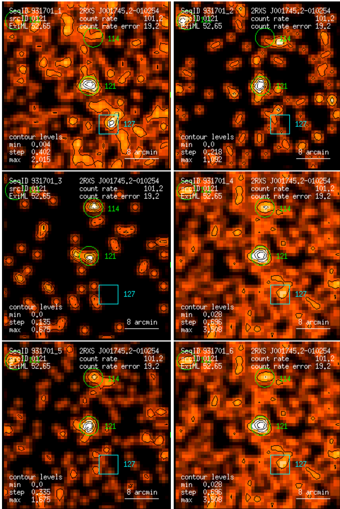
Figure 121: RASS 931701: detection 0121: band rate images, Gaussian filter: (1) PSPC channels 11 – 41, (2) 52 – 90, (3) 91 – 201, (4) 11 – 235, (5) 52 – 201, (6) 11 – 201. Broad band rates in counts/ks. Band rate contour levels in counts/ks/arcmin 2 .
