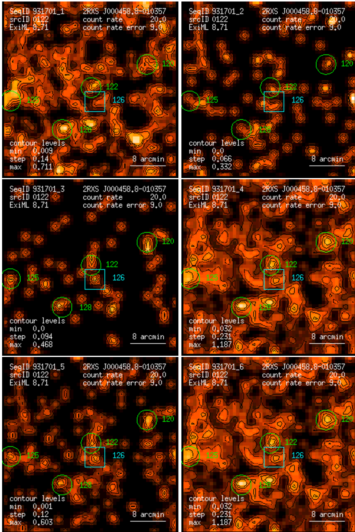
Figure 122: RASS 931701: detection 0122: band rate images, Gaussian filter: (1) PSPC channels 11 – 41, (2) 52 – 90, (3) 91 – 201, (4) 11 – 235, (5) 52 – 201, (6) 11 – 201. Broad band rates in counts/ks. Band rate contour levels in counts/ks/arcmin 2 .
