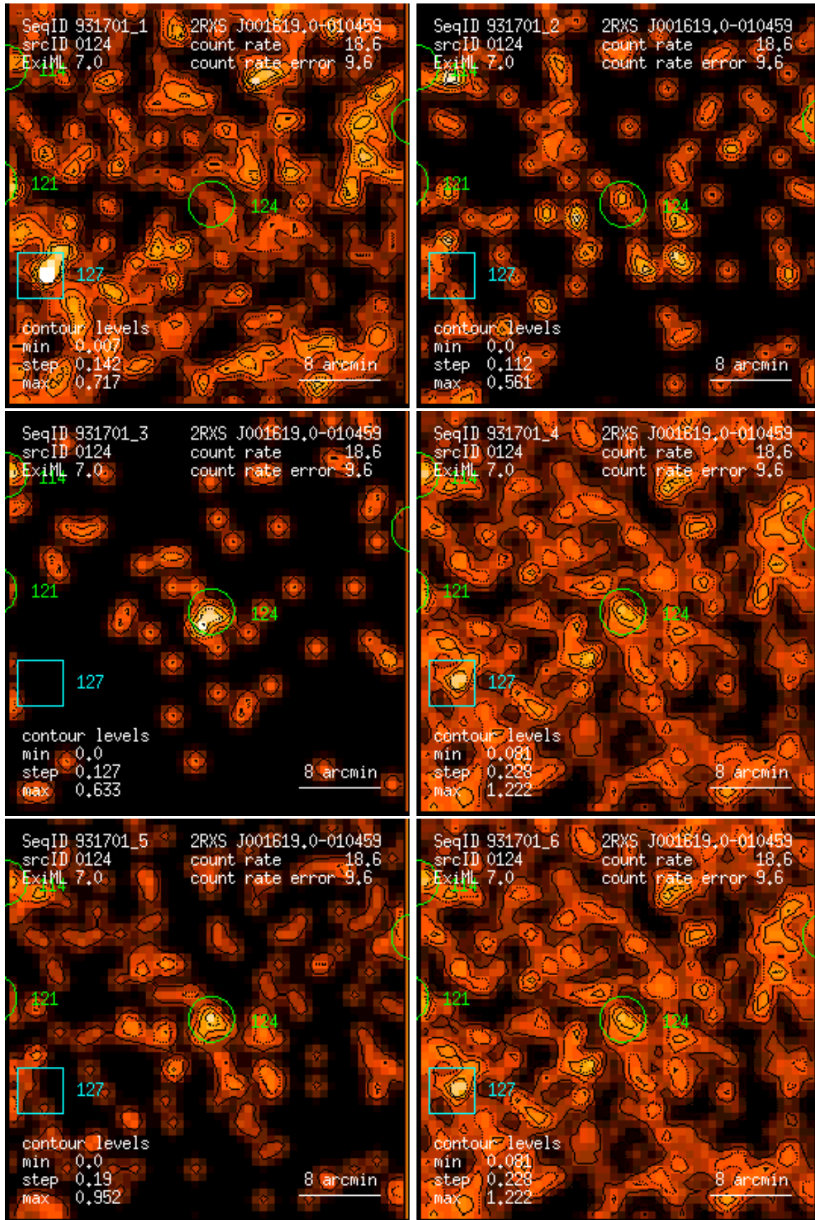
Figure 124: RASS 931701: detection 0124: band rate images, Gaussian filter: (1) PSPC channels 11 – 41, (2) 52 – 90, (3) 91 – 201, (4) 11 – 235, (5) 52 – 201, (6) 11 – 201. Broad band rates in counts/ks. Band rate contour levels in counts/ks/arcmin 2 .
