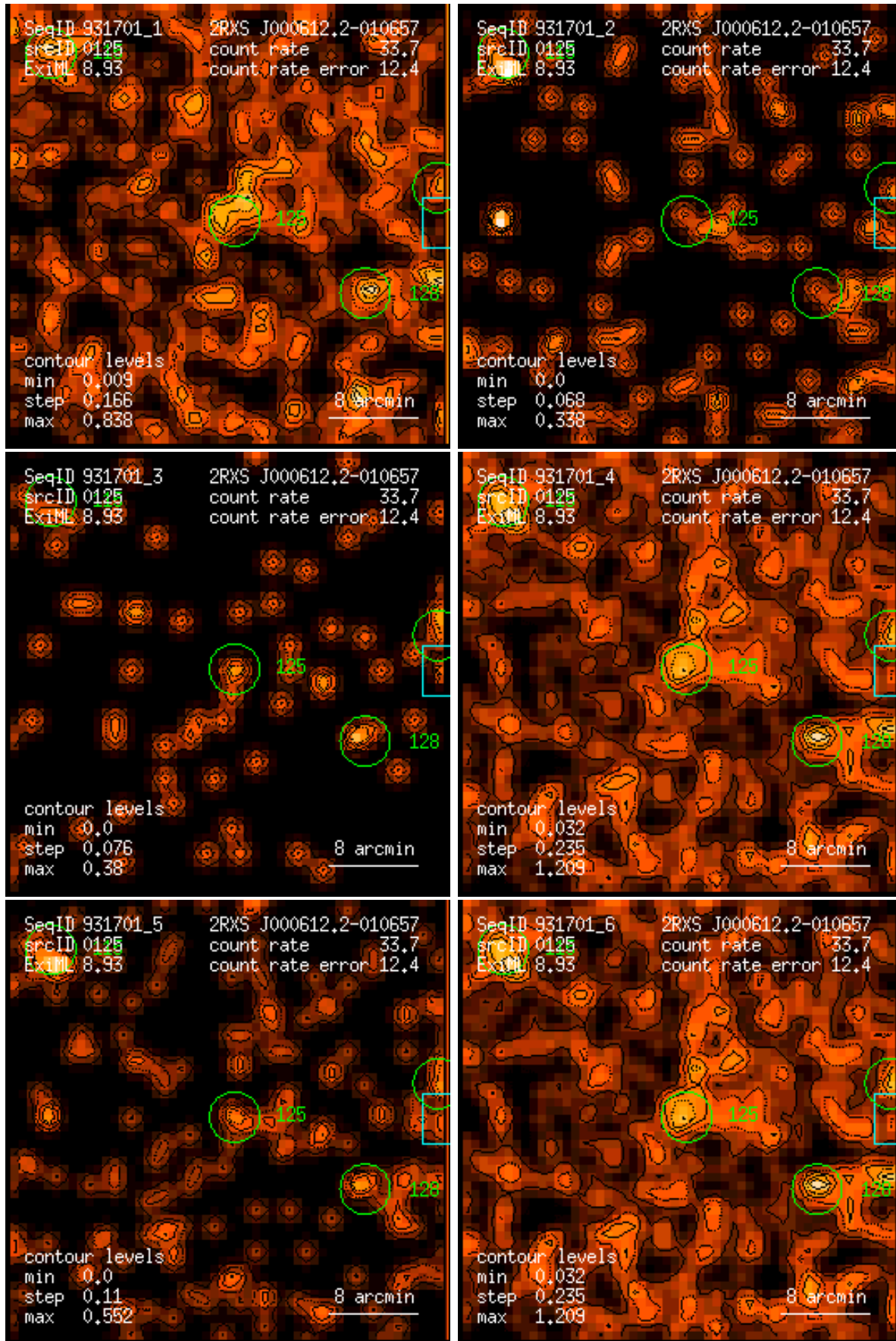
Figure 125: RASS 931701: detection 0125: band rate images, Gaussian filter: (1) PSPC channels 11 – 41, (2) 52 – 90, (3) 91 – 201, (4) 11 – 235, (5) 52 – 201, (6) 11 – 201. Broad band rates in counts/ks. Band rate contour levels in counts/ks/arcmin 2 .
