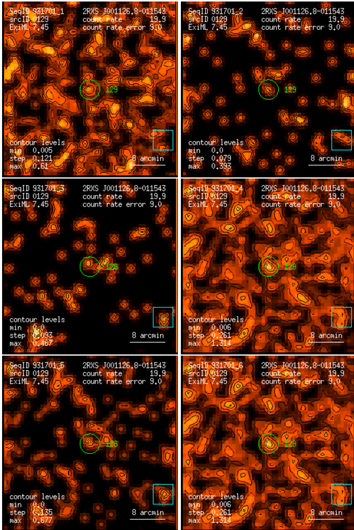
Figure 129: RASS 931701: detection 0129: band rate images, Gaussian filter: (1) PSPC channels 11 – 41, (2) 52 – 90, (3) 91 – 201, (4) 11 – 235, (5) 52 – 201, (6) 11 – 201. Broad band rates in counts/ks. Band rate contour levels in counts/ks/arcmin 2 .
