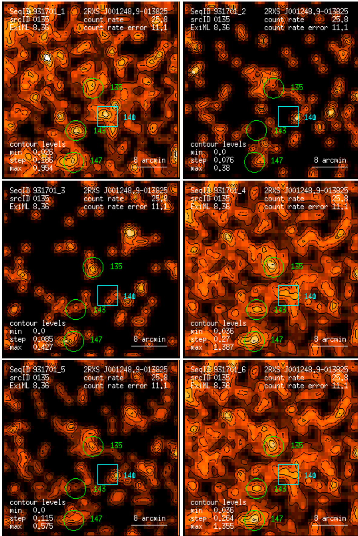
Figure 135: RASS 931701: detection 0135: band rate images, Gaussian filter: (1) PSPC channels 11 – 41, (2) 52 – 90, (3) 91 – 201, (4) 11 – 235, (5) 52 – 201, (6) 11 – 201. Broad band rates in counts/ks. Band rate contour levels in counts/ks/arcmin 2 .
