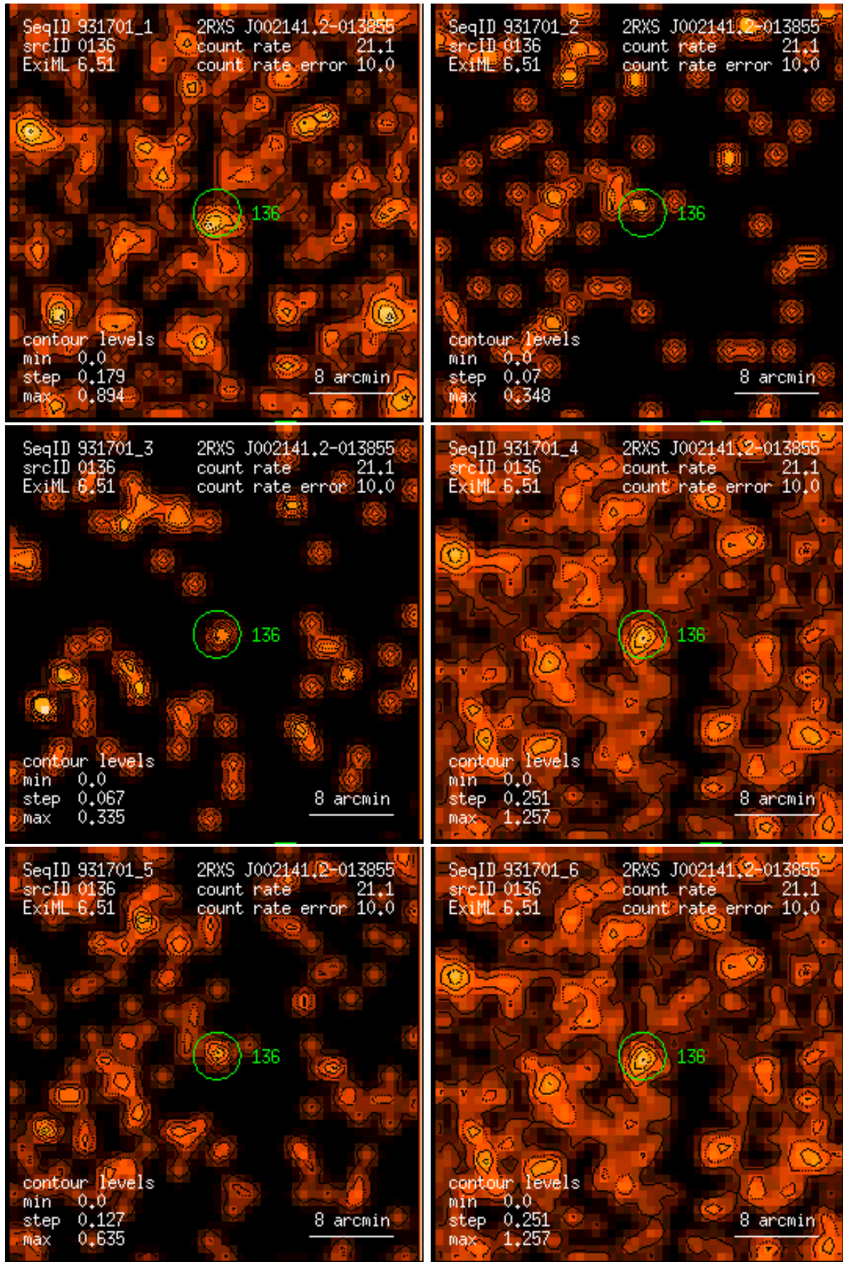
Figure 136: RASS 931701: detection 0136: band rate images, Gaussian filter: (1) PSPC channels 11 – 41, (2) 52 – 90, (3) 91 – 201, (4) 11 – 235, (5) 52 – 201, (6) 11 – 201. Broad band rates in counts/ks. Band rate contour levels in counts/ks/arcmin 2 .
