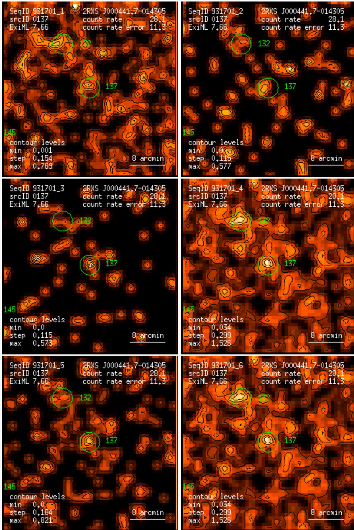
Figure 137: RASS 931701: detection 0137: band rate images, Gaussian filter: (1) PSPC channels 11 – 41, (2) 52 – 90, (3) 91 – 201, (4) 11 – 235, (5) 52 – 201, (6) 11 – 201. Broad band rates in counts/ks. Band rate contour levels in counts/ks/arcmin 2 .
