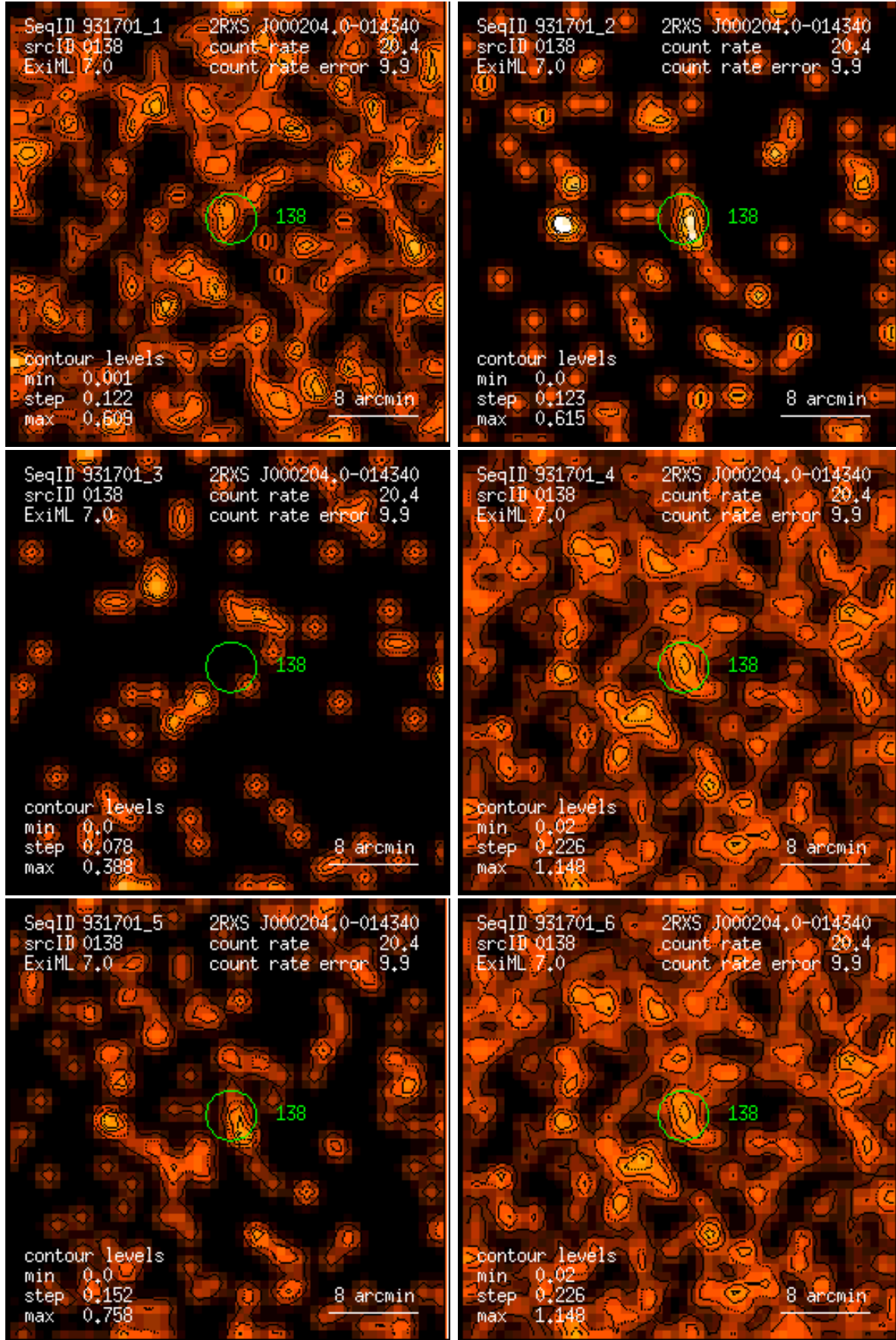
Figure 138: RASS 931701: detection 0138: band rate images, Gaussian filter: (1) PSPC channels 11 – 41, (2) 52 – 90, (3) 91 – 201, (4) 11 – 235, (5) 52 – 201, (6) 11 – 201. Broad band rates in counts/ks. Band rate contour levels in counts/ks/arcmin 2 .
