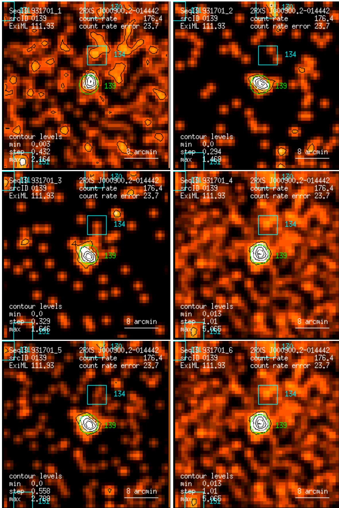
Figure 139: RASS 931701: detection 0139: band rate images, Gaussian filter: (1) PSPC channels 11 – 41, (2) 52 – 90, (3) 91 – 201, (4) 11 – 235, (5) 52 – 201, (6) 11 – 201. Broad band rates in counts/ks. Band rate contour levels in counts/ks/arcmin 2 .
