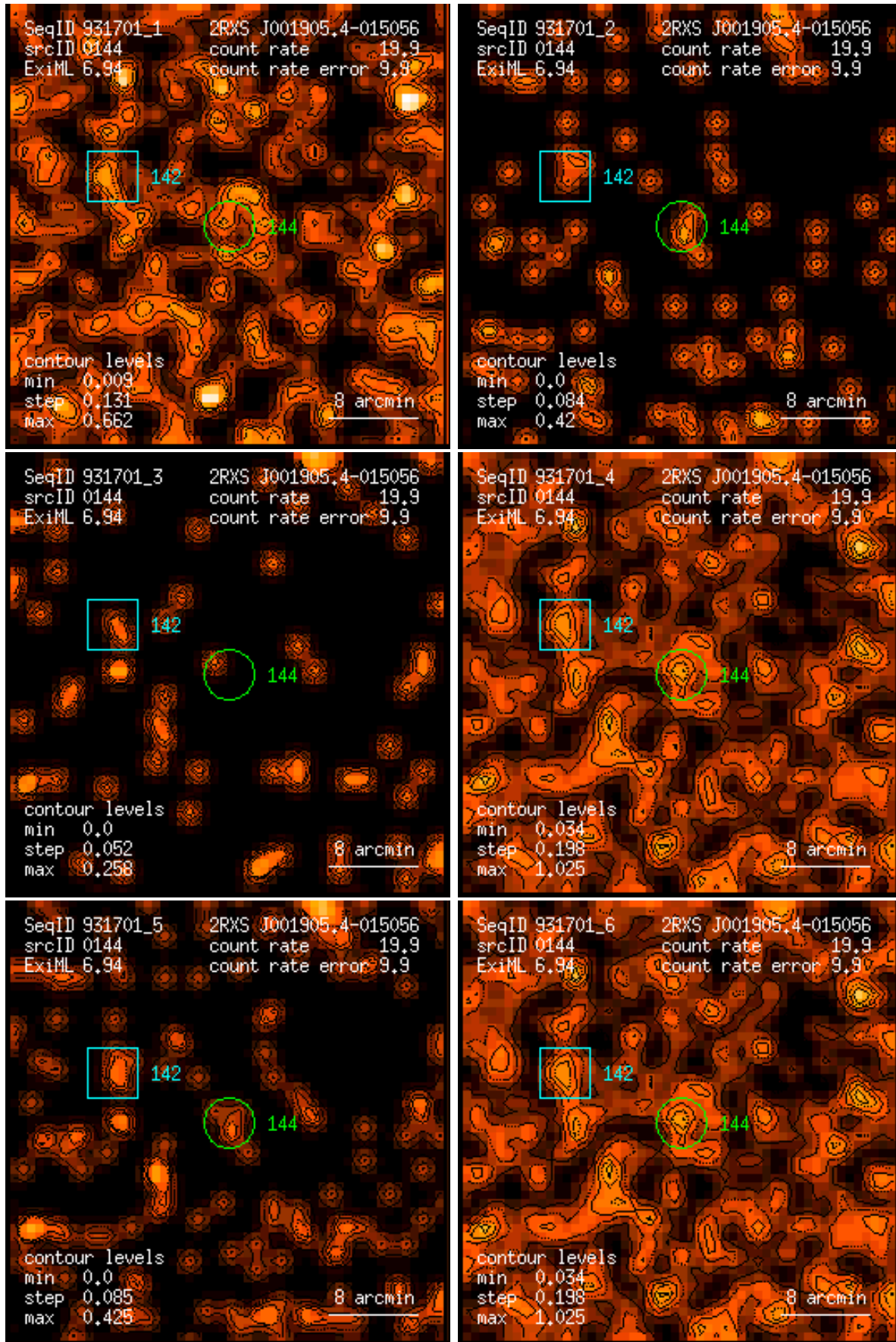
Figure 144: RASS 931701: detection 0144: band rate images, Gaussian filter: (1) PSPC channels 11 – 41, (2) 52 – 90, (3) 91 – 201, (4) 11 – 235, (5) 52 – 201, (6) 11 – 201. Broad band rates in counts/ks. Band rate contour levels in counts/ks/arcmin 2 .
