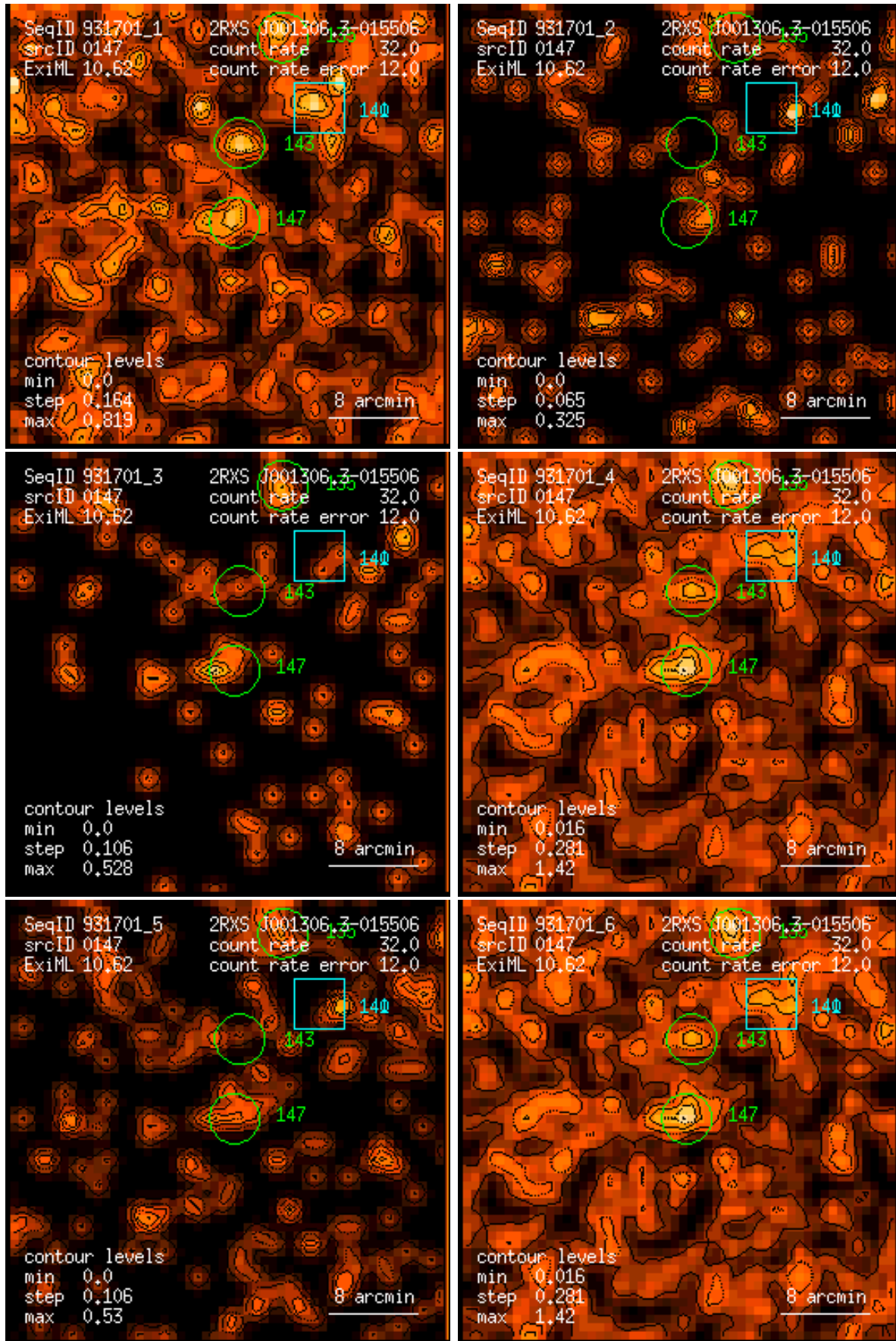
Figure 147: RASS 931701: detection 0147: band rate images, Gaussian filter: (1) PSPC channels 11 – 41, (2) 52 – 90, (3) 91 – 201, (4) 11 – 235, (5) 52 – 201, (6) 11 – 201. Broad band rates in counts/ks. Band rate contour levels in counts/ks/arcmin 2 .
