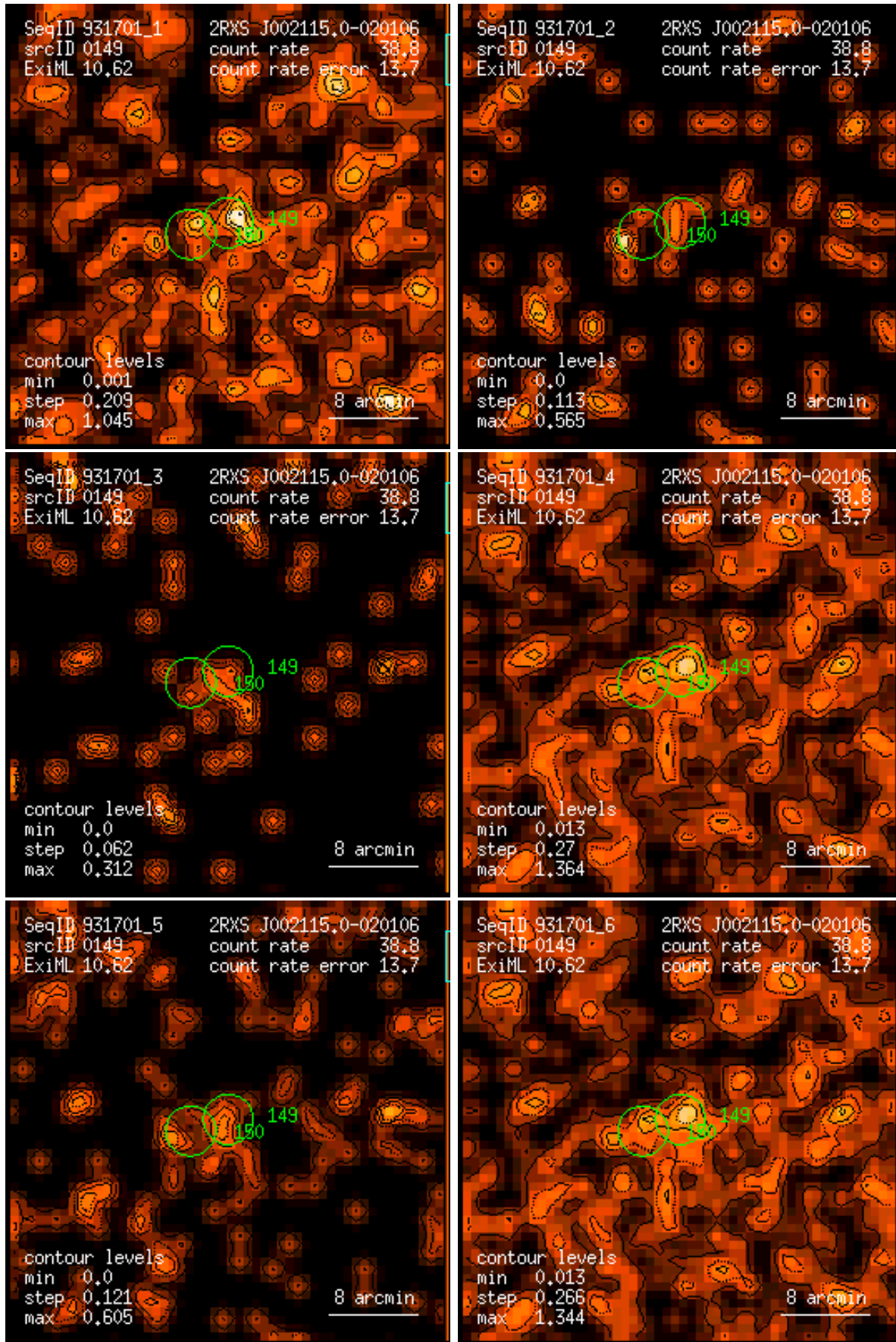
Figure 149: RASS 931701: detection 0149: band rate images, Gaussian filter: (1) PSPC channels 11 – 41, (2) 52 – 90, (3) 91 – 201, (4) 11 – 235, (5) 52 – 201, (6) 11 – 201. Broad band rates in counts/ks. Band rate contour levels in counts/ks/arcmin 2 .
