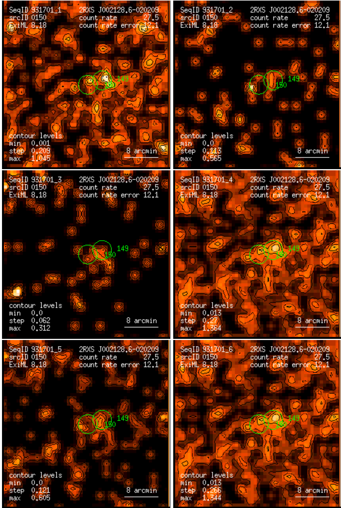
Figure 150: RASS 931701: detection 0150: band rate images, Gaussian filter: (1) PSPC channels 11 – 41, (2) 52 – 90, (3) 91 – 201, (4) 11 – 235, (5) 52 – 201, (6) 11 – 201. Broad band rates in counts/ks. Band rate contour levels in counts/ks/arcmin 2 .
