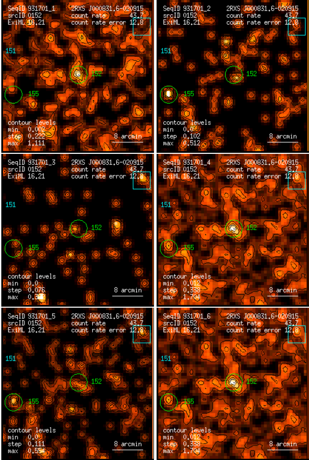
Figure 152: RASS 931701: detection 0152: band rate images, Gaussian filter: (1) PSPC channels 11 – 41, (2) 52 – 90, (3) 91 – 201, (4) 11 – 235, (5) 52 – 201, (6) 11 – 201. Broad band rates in counts/ks. Band rate contour levels in counts/ks/arcmin 2 .
