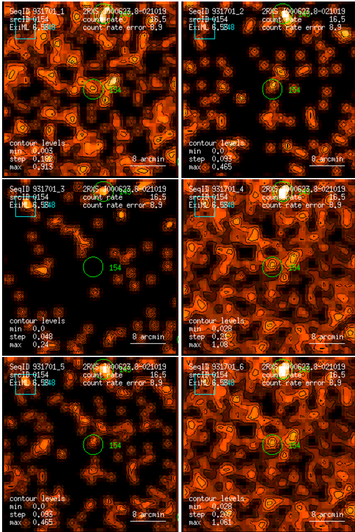
Figure 154: RASS 931701: detection 0154: band rate images, Gaussian filter: (1) PSPC channels 11 – 41, (2) 52 – 90, (3) 91 – 201, (4) 11 – 235, (5) 52 – 201, (6) 11 – 201. Broad band rates in counts/ks. Band rate contour levels in counts/ks/arcmin 2 .
