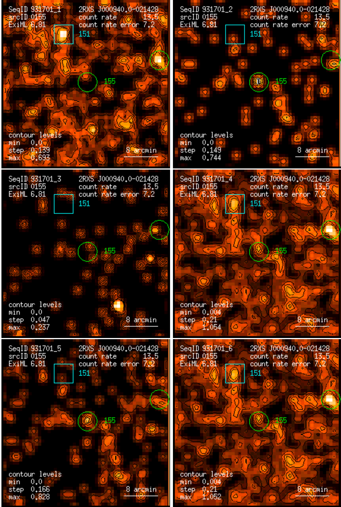
Figure 155: RASS 931701: detection 0155: band rate images, Gaussian filter: (1) PSPC channels 11 – 41, (2) 52 – 90, (3) 91 – 201, (4) 11 – 235, (5) 52 – 201, (6) 11 – 201. Broad band rates in counts/ks. Band rate contour levels in counts/ks/arcmin 2 .
