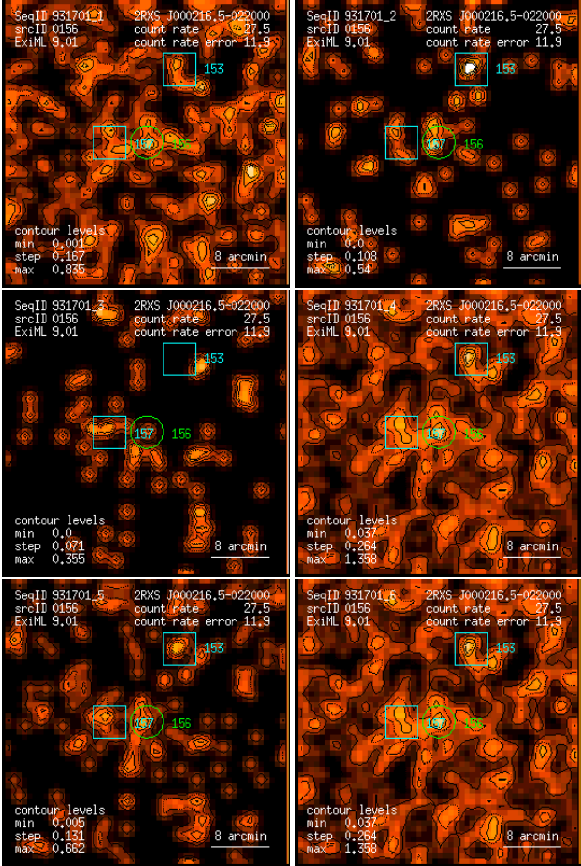
Figure 156: RASS 931701: detection 0156: band rate images, Gaussian filter: (1) PSPC channels 11 – 41, (2) 52 – 90, (3) 91 – 201, (4) 11 – 235, (5) 52 – 201, (6) 11 – 201. Broad band rates in counts/ks. Band rate contour levels in counts/ks/arcmin 2 .
