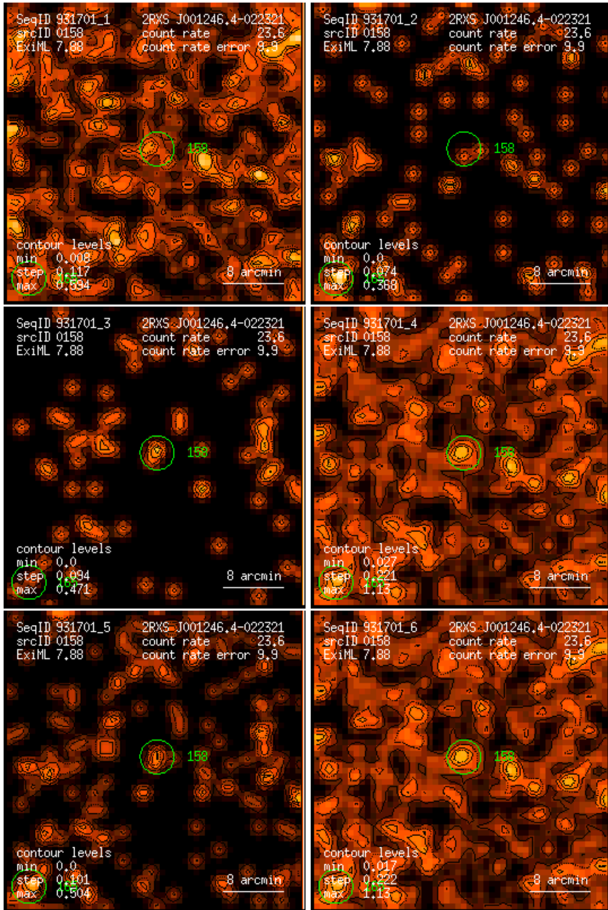
Figure 158: RASS 931701: detection 0158: band rate images, Gaussian filter: (1) PSPC channels 11 – 41, (2) 52 – 90, (3) 91 – 201, (4) 11 – 235, (5) 52 – 201, (6) 11 – 201. Broad band rates in counts/ks. Band rate contour levels in counts/ks/arcmin 2 .
