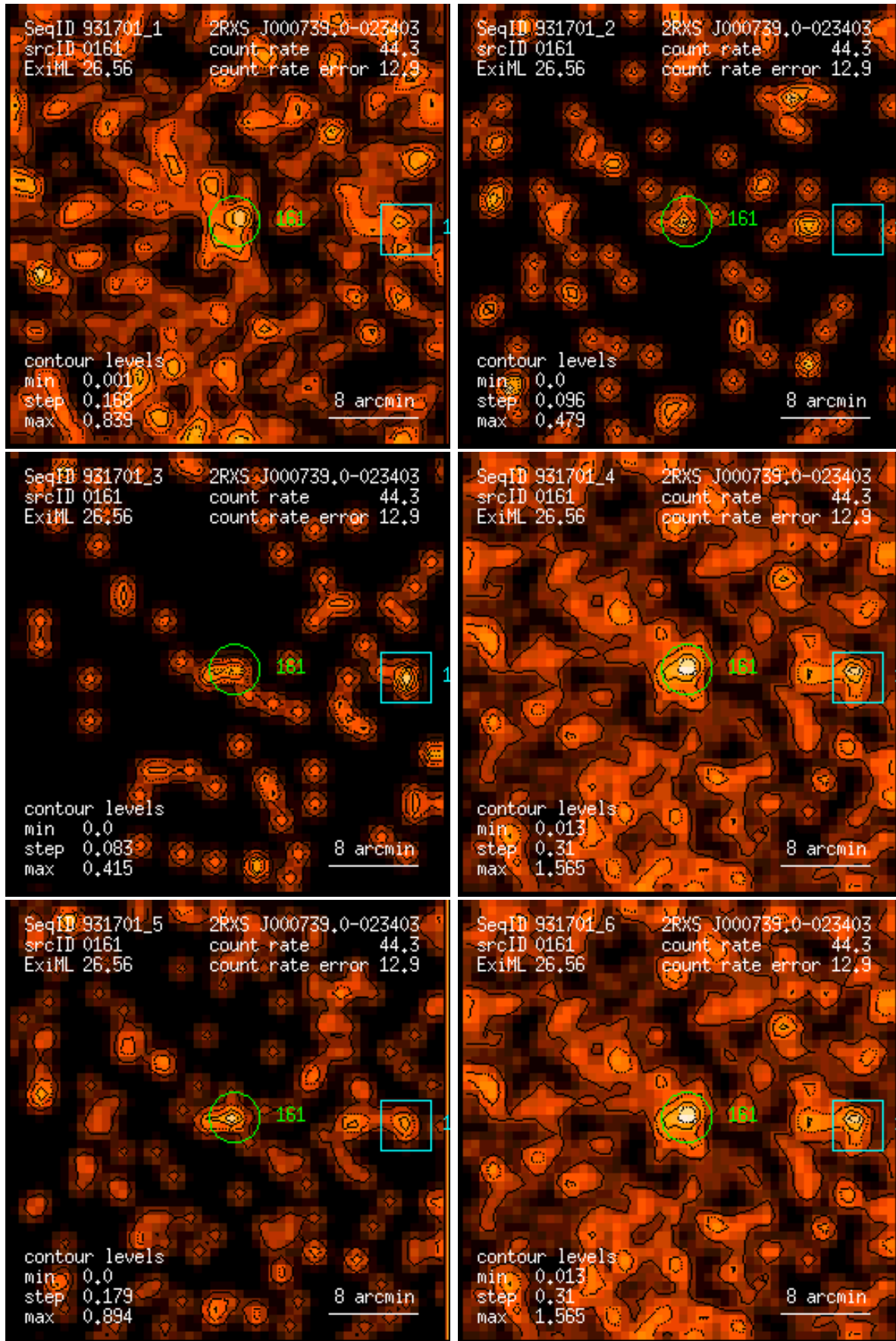
Figure 161: RASS 931701: detection 0161: band rate images, Gaussian filter: (1) PSPC channels 11 – 41, (2) 52 – 90, (3) 91 – 201, (4) 11 – 235, (5) 52 – 201, (6) 11 – 201. Broad band rates in counts/ks. Band rate contour levels in counts/ks/arcmin 2 .
