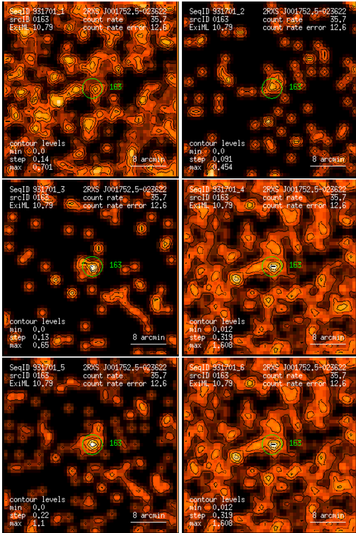
Figure 163: RASS 931701: detection 0163: band rate images, Gaussian filter: (1) PSPC channels 11 – 41, (2) 52 – 90, (3) 91 – 201, (4) 11 – 235, (5) 52 – 201, (6) 11 – 201. Broad band rates in counts/ks. Band rate contour levels in counts/ks/arcmin 2 .
