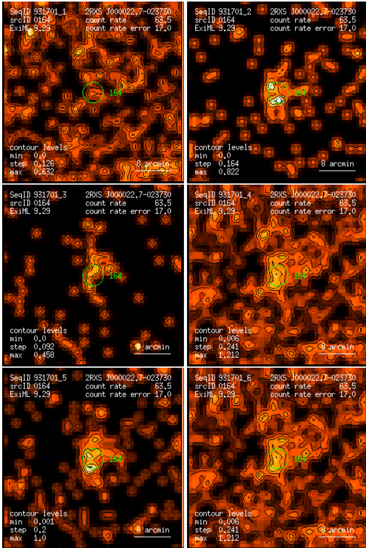
Figure 164: RASS 931701: detection 0164: band rate images, Gaussian filter: (1) PSPC channels 11 – 41, (2) 52 – 90, (3) 91 – 201, (4) 11 – 235, (5) 52 – 201, (6) 11 – 201. Broad band rates in counts/ks. Band rate contour levels in counts/ks/arcmin 2 .
