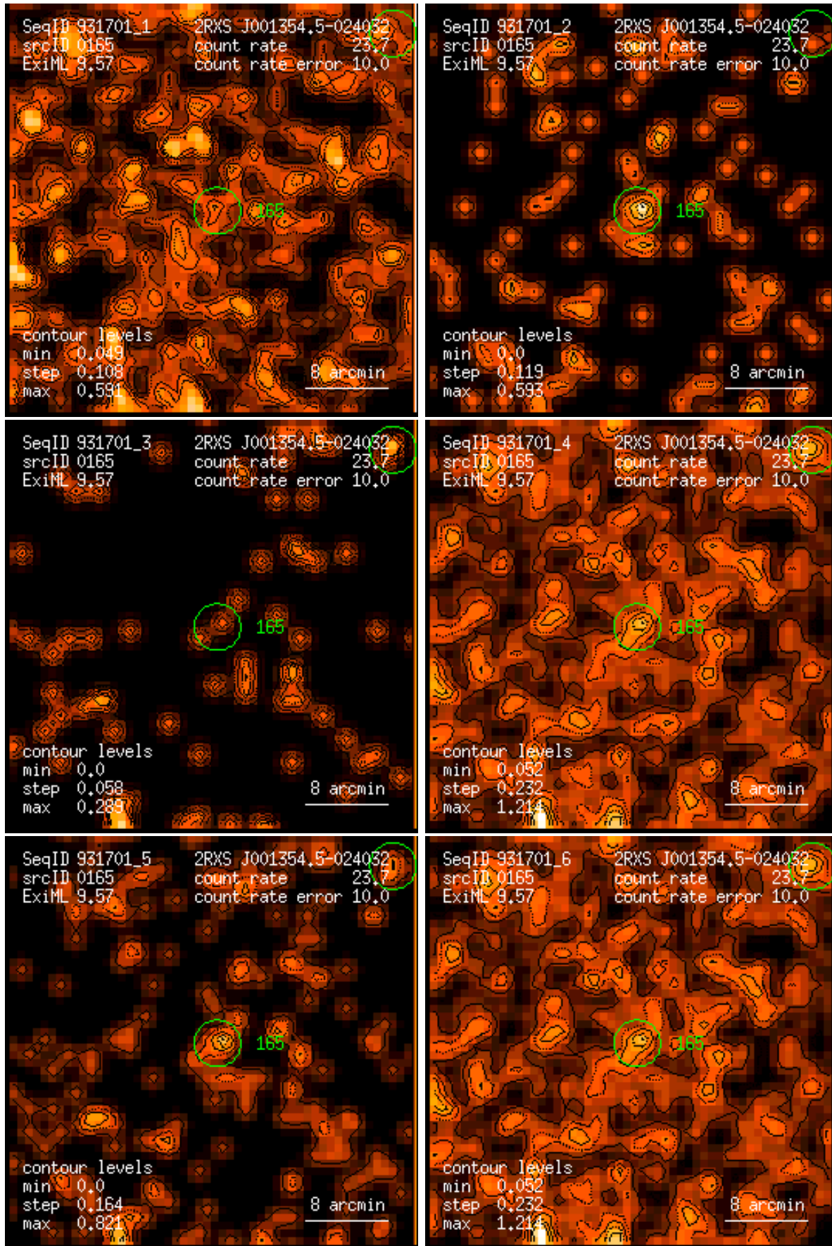
Figure 165: RASS 931701: detection 0165: band rate images, Gaussian filter: (1) PSPC channels 11 – 41, (2) 52 – 90, (3) 91 – 201, (4) 11 – 235, (5) 52 – 201, (6) 11 – 201. Broad band rates in counts/ks. Band rate contour levels in counts/ks/arcmin 2 .
