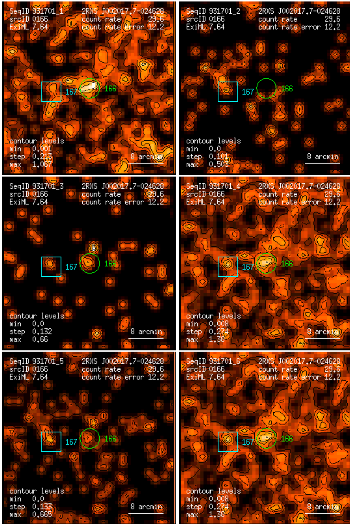
Figure 166: RASS 931701: detection 0166: band rate images, Gaussian filter: (1) PSPC channels 11 – 41, (2) 52 – 90, (3) 91 – 201, (4) 11 – 235, (5) 52 – 201, (6) 11 – 201. Broad band rates in counts/ks. Band rate contour levels in counts/ks/arcmin 2 .
