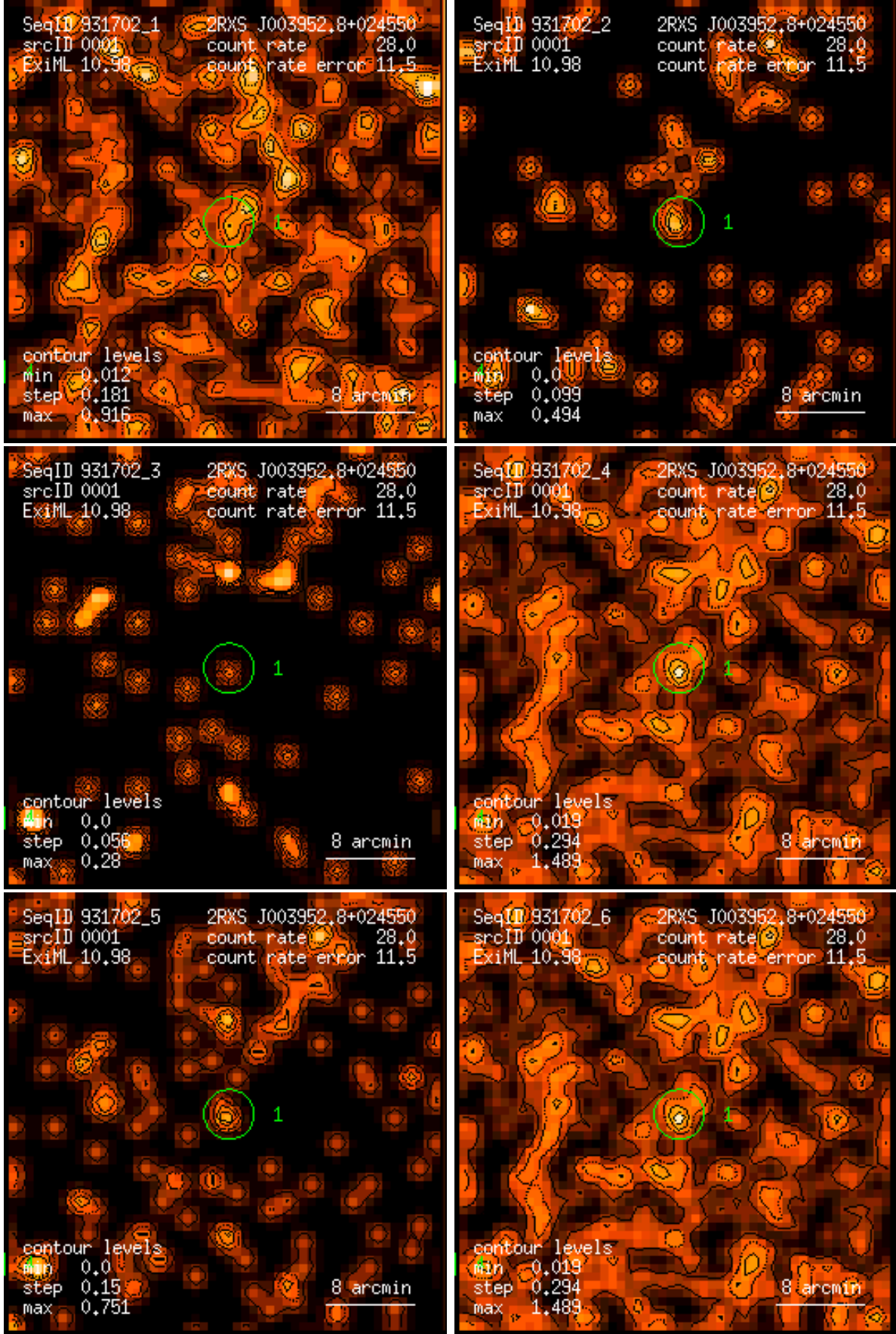
Figure 1: RASS 931702: detection 0001: band rate images, Gaussian filter: (1) PSPC channels 11 – 41, (2) 52 – 90, (3) 91 – 201, (4) 11 – 235, (5) 52 – 201, (6) 11 – 201. Broad band rates in counts/ks. Band rate contour levels in counts/ks/arcmin 2 .
