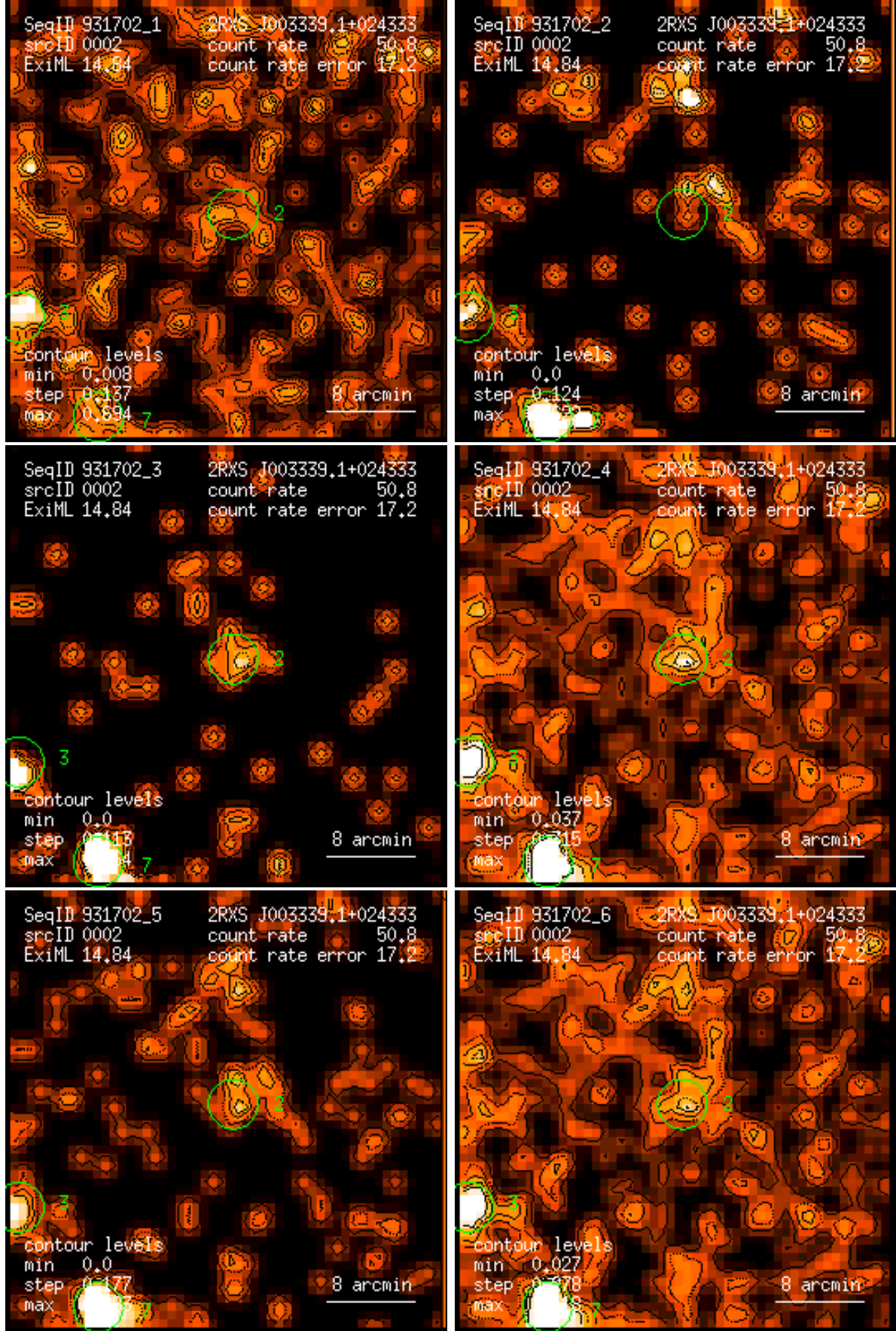
Figure 2: RASS 931702: detection 0002: band rate images, Gaussian filter: (1) PSPC channels 11 – 41, (2) 52 – 90, (3) 91 – 201, (4) 11 – 235, (5) 52 – 201, (6) 11 – 201. Broad band rates in counts/ks. Band rate contour levels in counts/ks/arcmin 2 .
