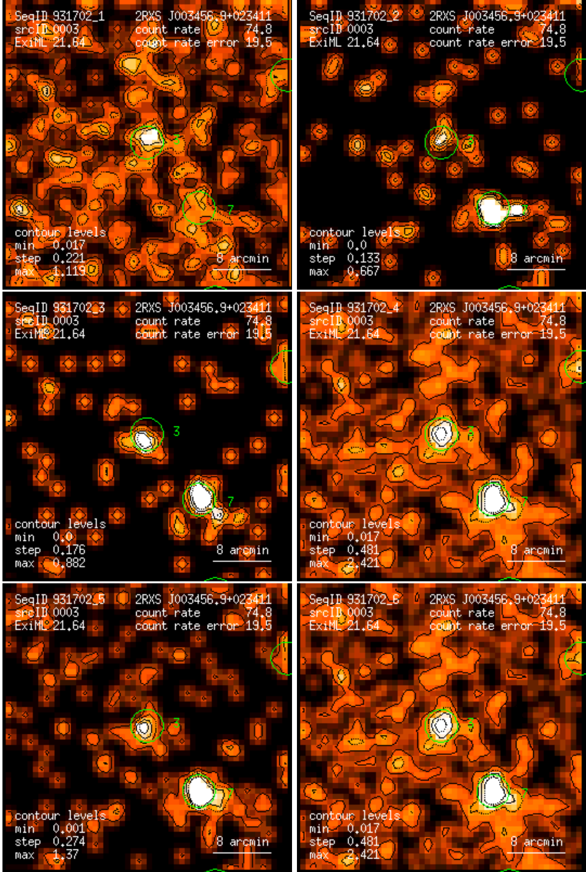
Figure 3: RASS 931702: detection 0003: band rate images, Gaussian filter: (1) PSPC channels 11 – 41, (2) 52 – 90, (3) 91 – 201, (4) 11 – 235, (5) 52 – 201, (6) 11 – 201. Broad band rates in counts/ks. Band rate contour levels in counts/ks/arcmin 2 .
