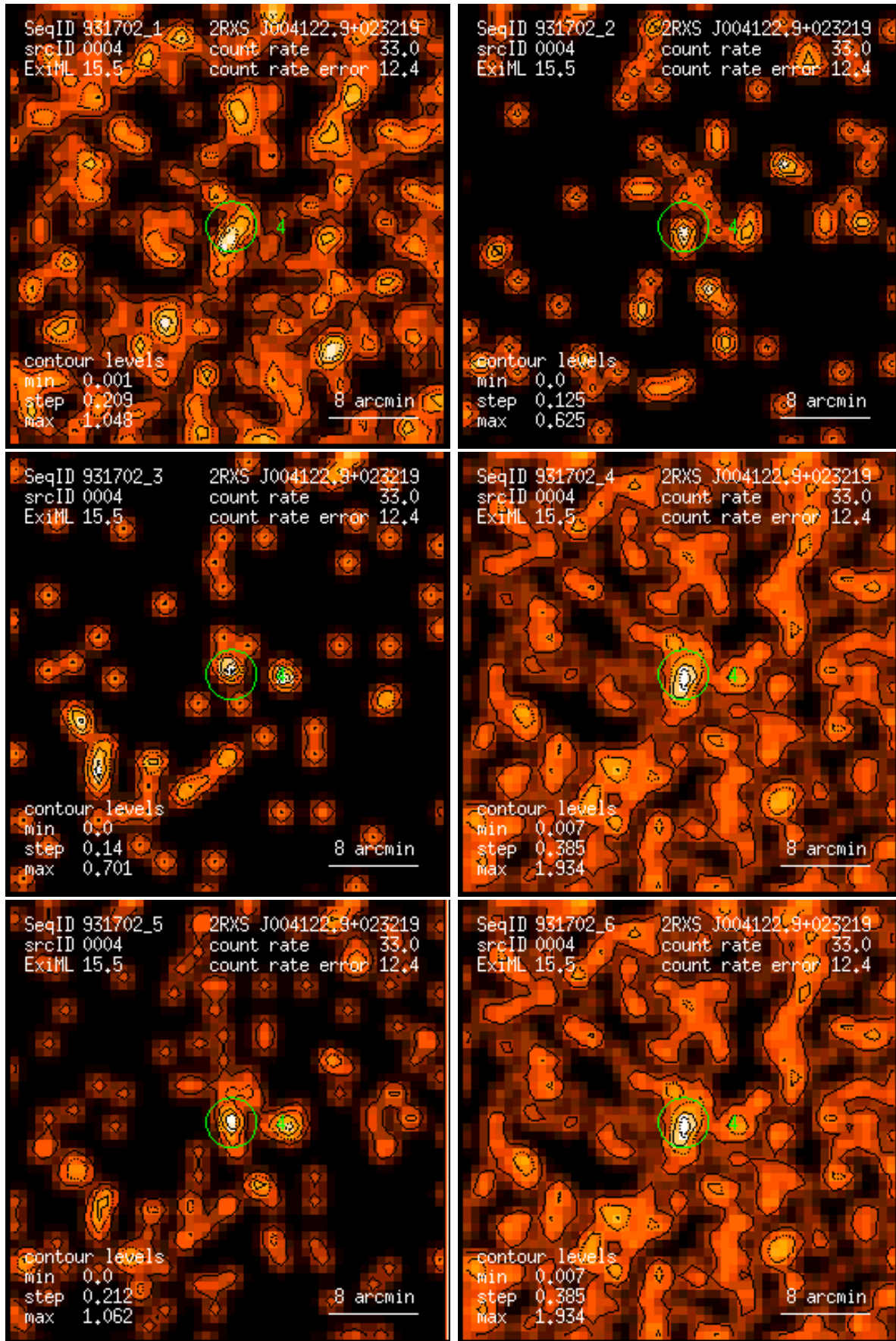
Figure 4: RASS 931702: detection 0004: band rate images, Gaussian filter: (1) PSPC channels 11 – 41, (2) 52 – 90, (3) 91 – 201, (4) 11 – 235, (5) 52 – 201, (6) 11 – 201. Broad band rates in counts/ks. Band rate contour levels in counts/ks/arcmin 2 .
