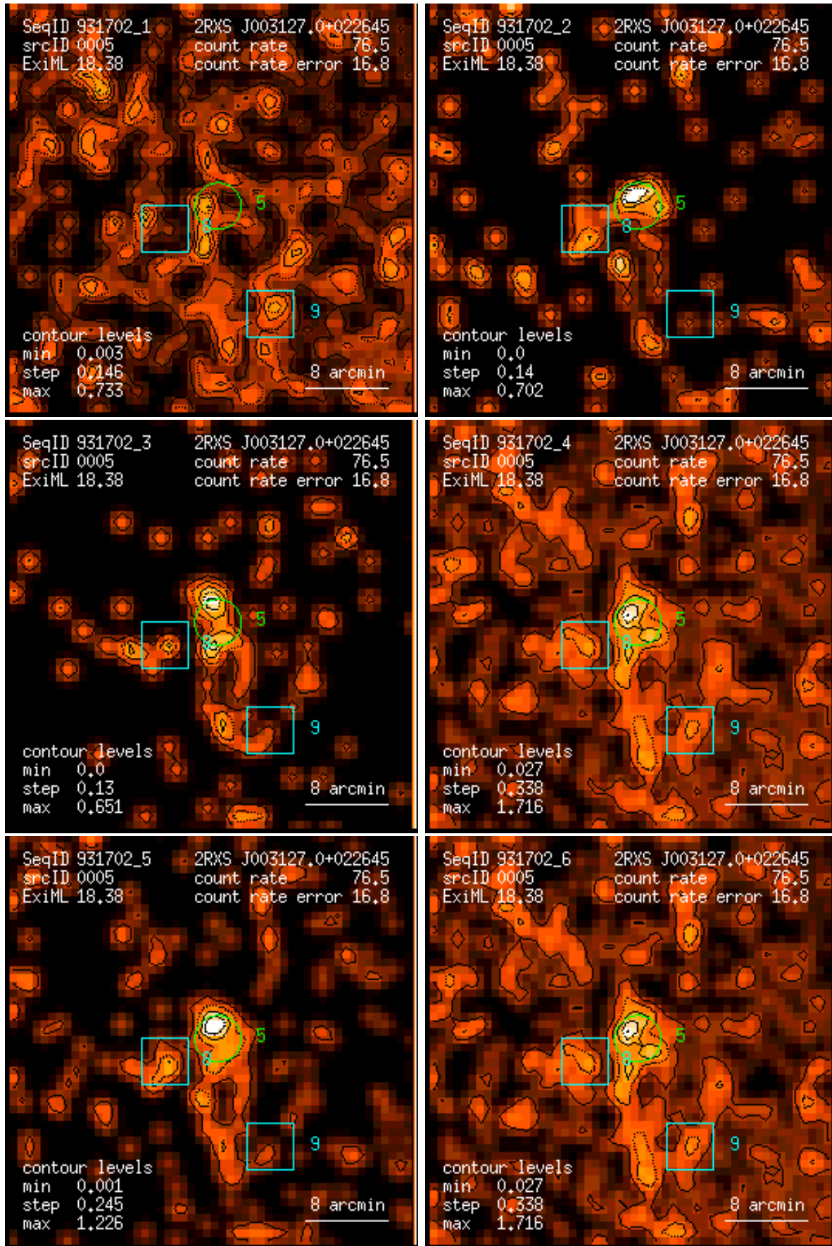
Figure 5: RASS 931702: detection 0005: band rate images, Gaussian filter: (1) PSPC channels 11 – 41, (2) 52 – 90, (3) 91 – 201, (4) 11 – 235, (5) 52 – 201, (6) 11 – 201. Broad band rates in counts/ks. Band rate contour levels in counts/ks/arcmin 2 .
