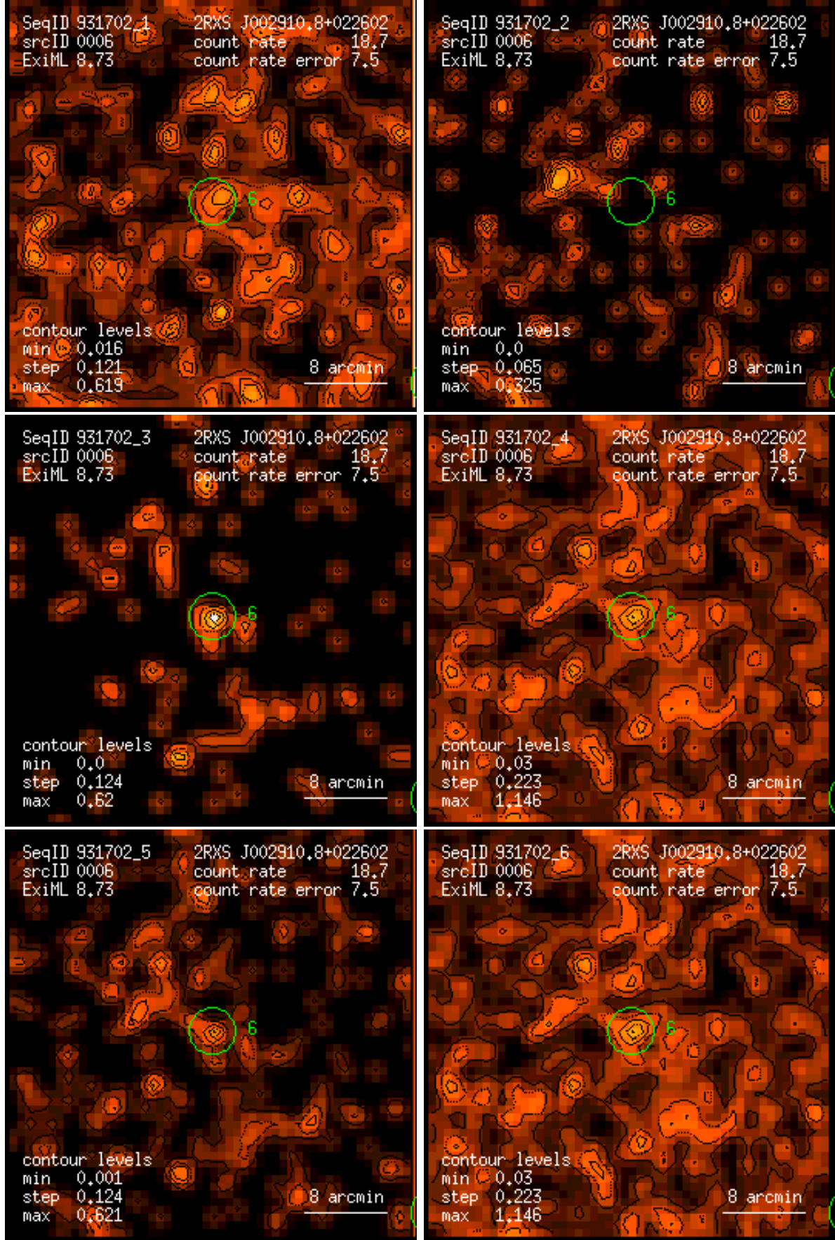
Figure 6: RASS 931702: detection 0006: band rate images, Gaussian filter: (1) PSPC channels 11 – 41, (2) 52 – 90, (3) 91 – 201, (4) 11 – 235, (5) 52 – 201, (6) 11 – 201. Broad band rates in counts/ks. Band rate contour levels in counts/ks/arcmin 2 .
