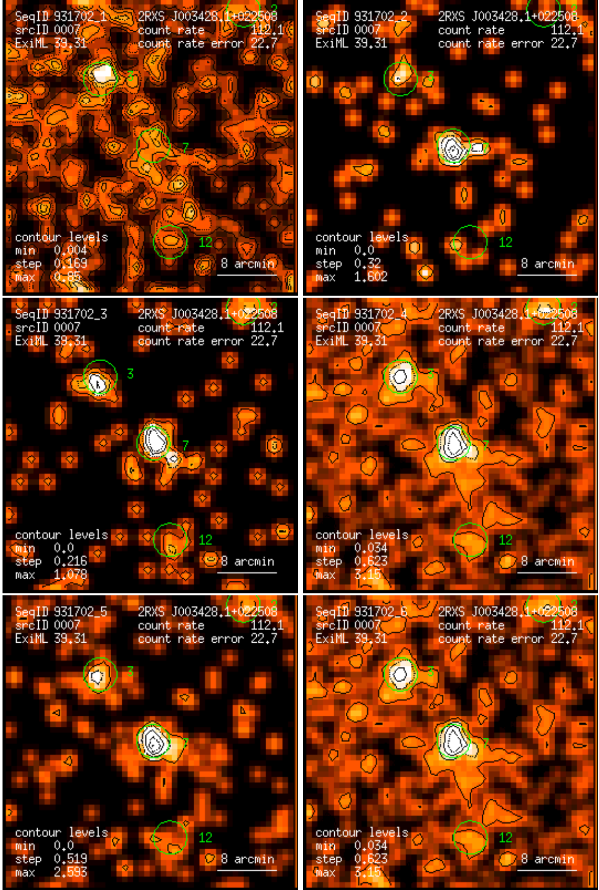
Figure 7: RASS 931702: detection 0007: band rate images, Gaussian filter: (1) PSPC channels 11 – 41, (2) 52 – 90, (3) 91 – 201, (4) 11 – 235, (5) 52 – 201, (6) 11 – 201. Broad band rates in counts/ks. Band rate contour levels in counts/ks/arcmin 2 .
