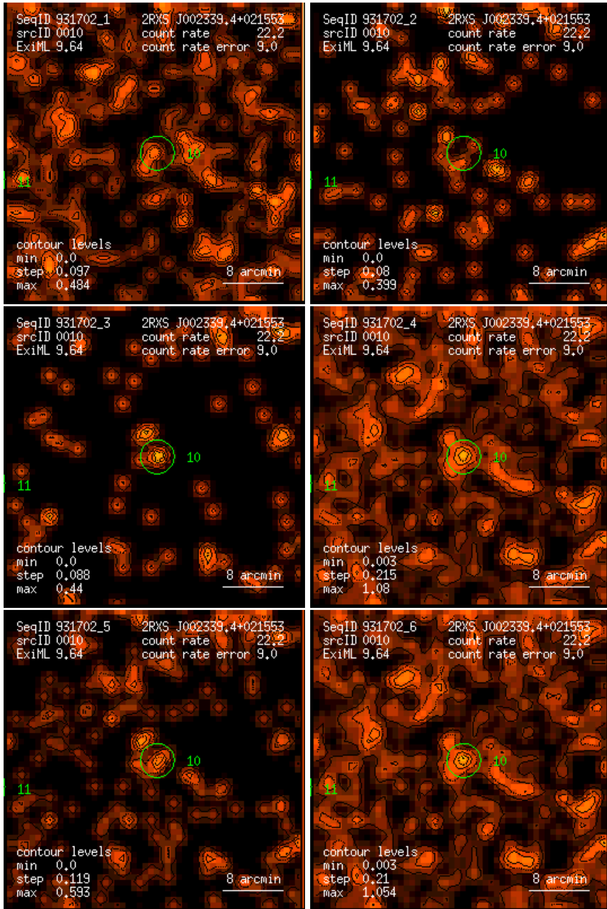
Figure 10: RASS 931702: detection 0010: band rate images, Gaussian filter: (1) PSPC channels 11 – 41, (2) 52 – 90, (3) 91 – 201, (4) 11 – 235, (5) 52 – 201, (6) 11 – 201. Broad band rates in counts/ks. Band rate contour levels in counts/ks/arcmin 2 .
