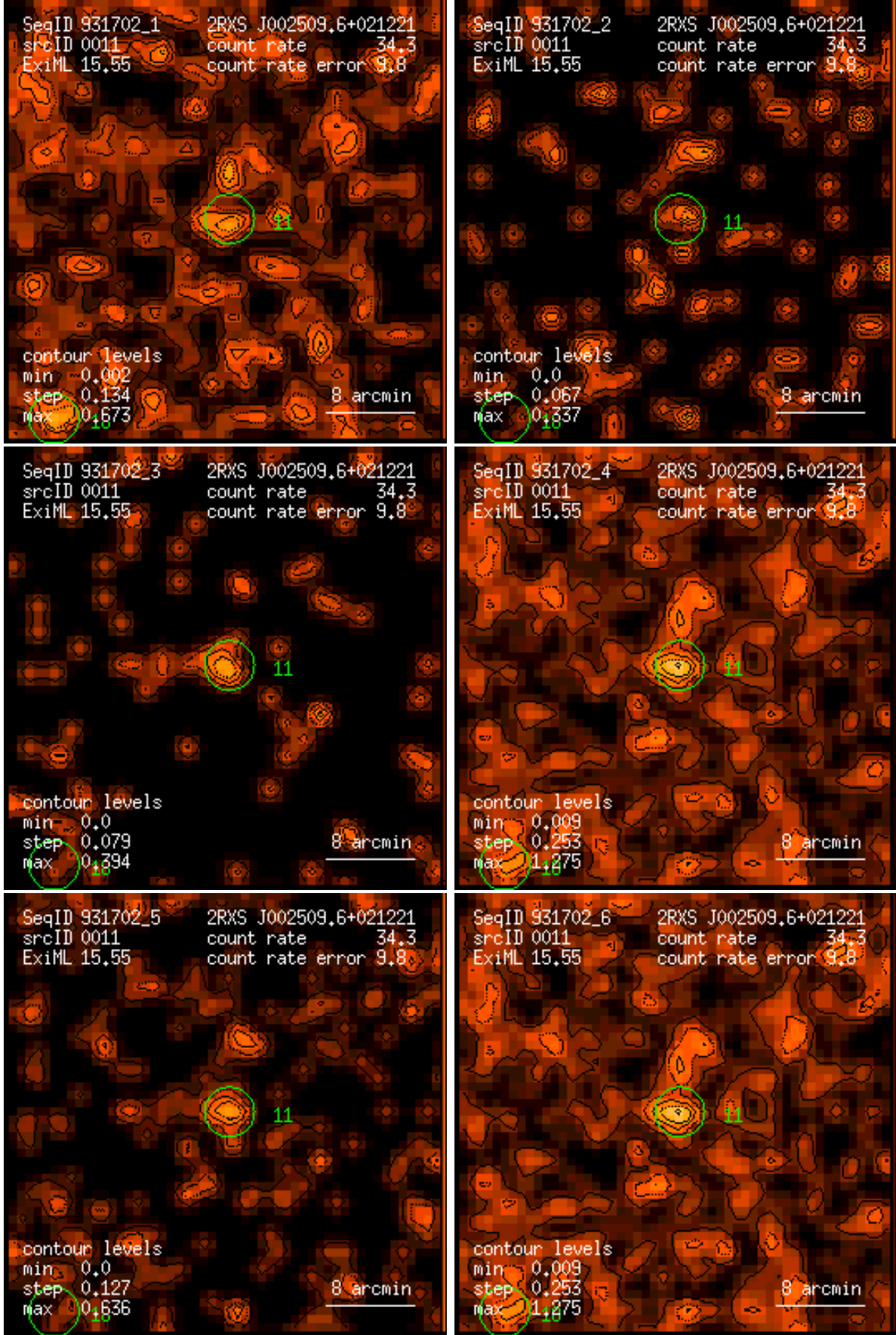
Figure 11: RASS 931702: detection 0011: band rate images, Gaussian filter: (1) PSPC channels 11 – 41, (2) 52 – 90, (3) 91 – 201, (4) 11 – 235, (5) 52 – 201, (6) 11 – 201. Broad band rates in counts/ks. Band rate contour levels in counts/ks/arcmin 2 .
