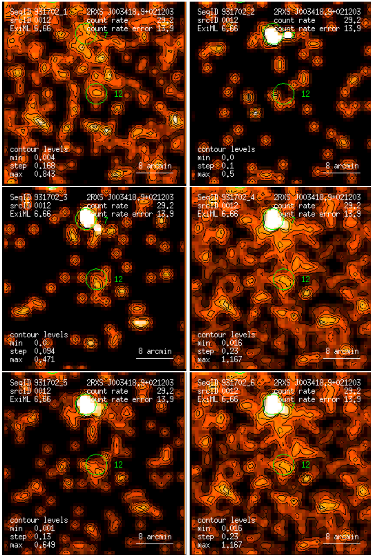
Figure 12: RASS 931702: detection 0012: band rate images, Gaussian filter: (1) PSPC channels 11 – 41, (2) 52 – 90, (3) 91 – 201, (4) 11 – 235, (5) 52 – 201, (6) 11 – 201. Broad band rates in counts/ks. Band rate contour levels in counts/ks/arcmin 2 .
