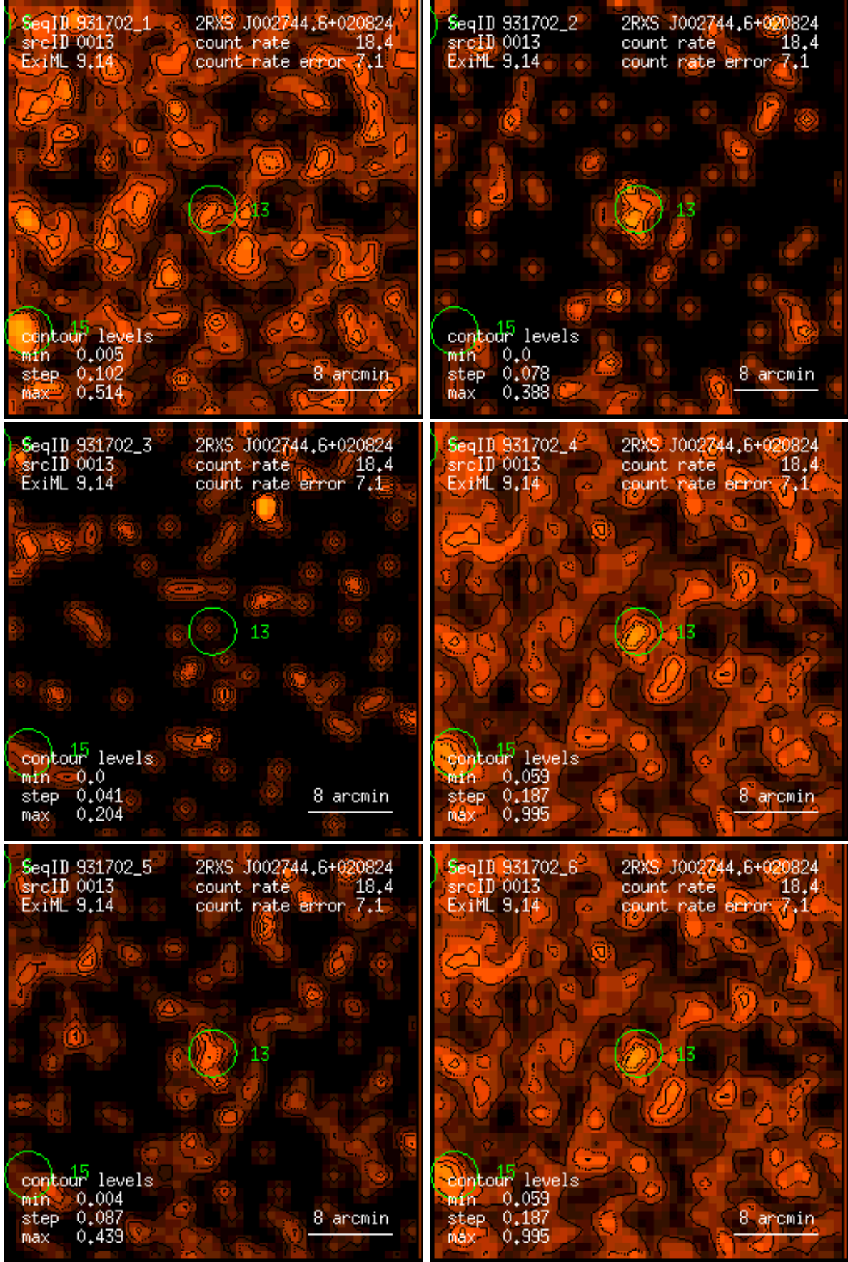
Figure 13: RASS 931702: detection 0013: band rate images, Gaussian filter: (1) PSPC channels 11 – 41, (2) 52 – 90, (3) 91 – 201, (4) 11 – 235, (5) 52 – 201, (6) 11 – 201. Broad band rates in counts/ks. Band rate contour levels in counts/ks/arcmin 2 .
