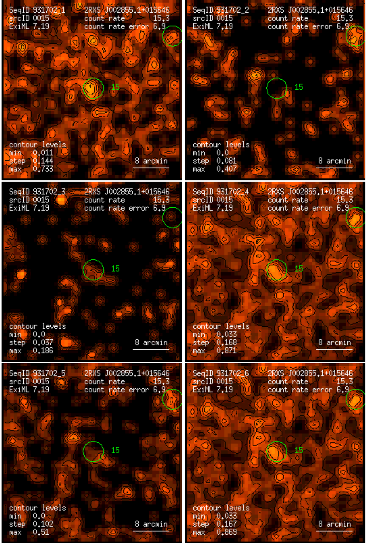
Figure 15: RASS 931702: detection 0015: band rate images, Gaussian filter: (1) PSPC channels 11 – 41, (2) 52 – 90, (3) 91 – 201, (4) 11 – 235, (5) 52 – 201, (6) 11 – 201. Broad band rates in counts/ks. Band rate contour levels in counts/ks/arcmin 2 .
