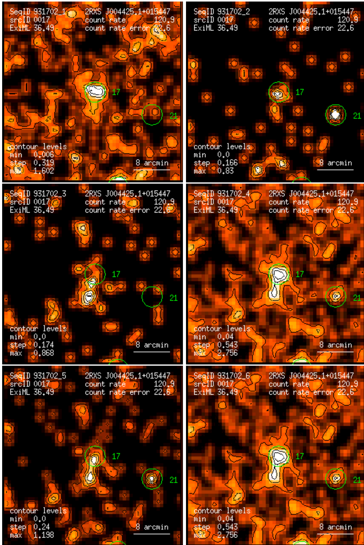
Figure 17: RASS 931702: detection 0017: band rate images, Gaussian filter: (1) PSPC channels 11 – 41, (2) 52 – 90, (3) 91 – 201, (4) 11 – 235, (5) 52 – 201, (6) 11 – 201. Broad band rates in counts/ks. Band rate contour levels in counts/ks/arcmin 2 .
