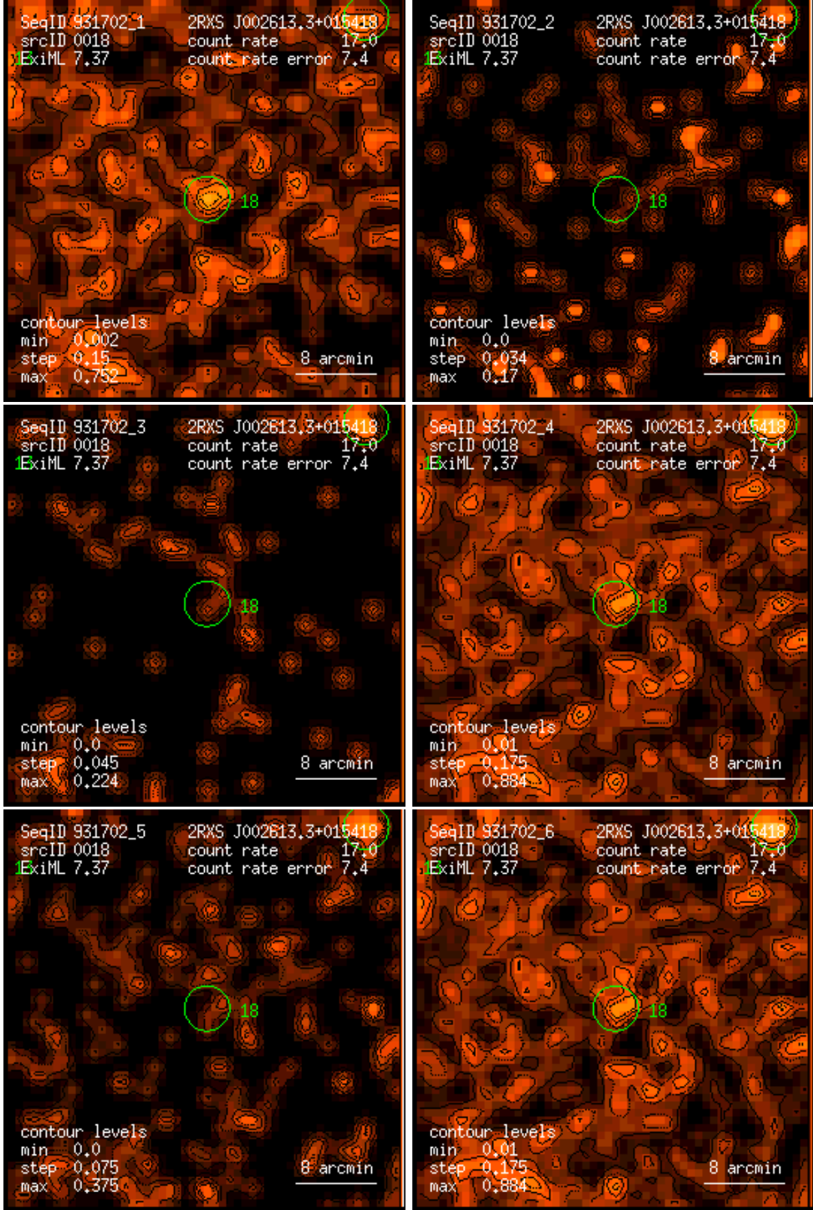
Figure 18: RASS 931702: detection 0018: band rate images, Gaussian filter: (1) PSPC channels 11 – 41, (2) 52 – 90, (3) 91 – 201, (4) 11 – 235, (5) 52 – 201, (6) 11 – 201. Broad band rates in counts/ks. Band rate contour levels in counts/ks/arcmin 2 .
