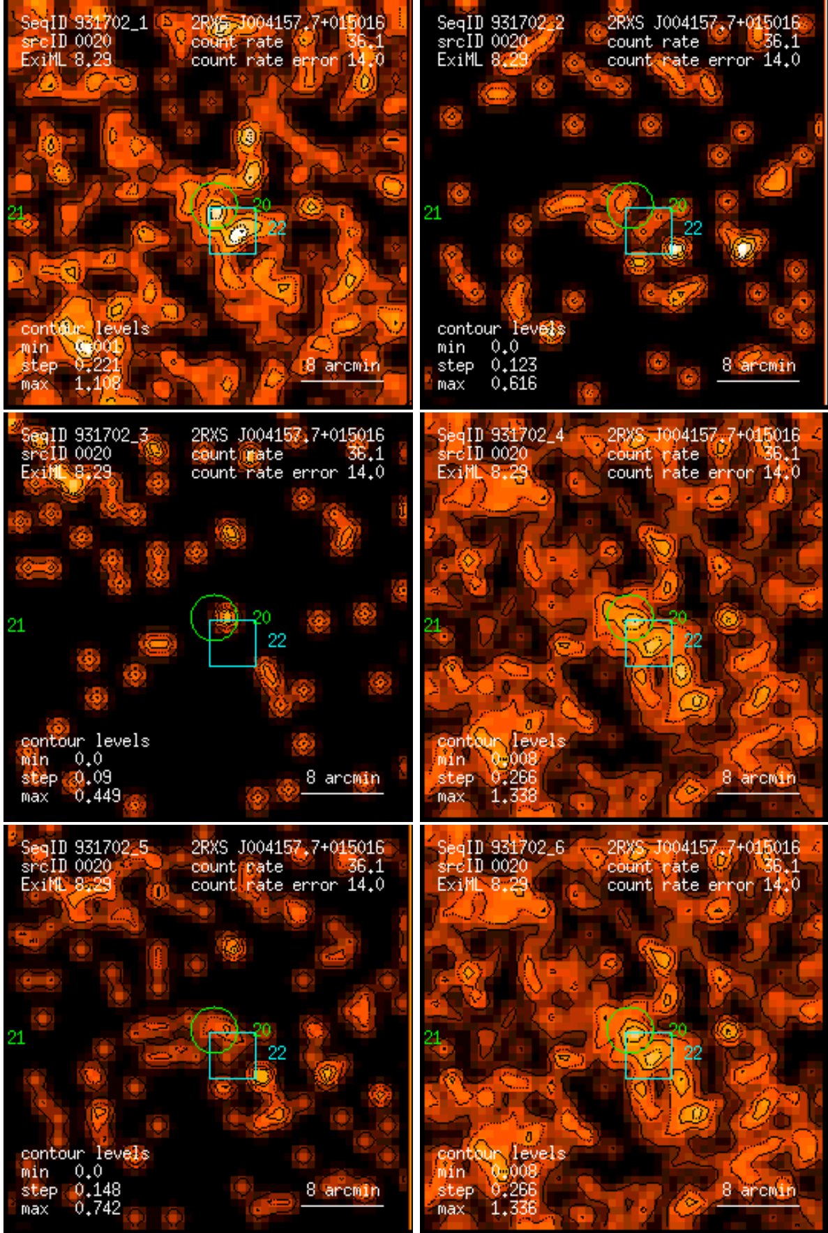
Figure 20: RASS 931702: detection 0020: band rate images, Gaussian filter: (1) PSPC channels 11 – 41, (2) 52 – 90, (3) 91 – 201, (4) 11 – 235, (5) 52 – 201, (6) 11 – 201. Broad band rates in counts/ks. Band rate contour levels in counts/ks/arcmin 2 .
