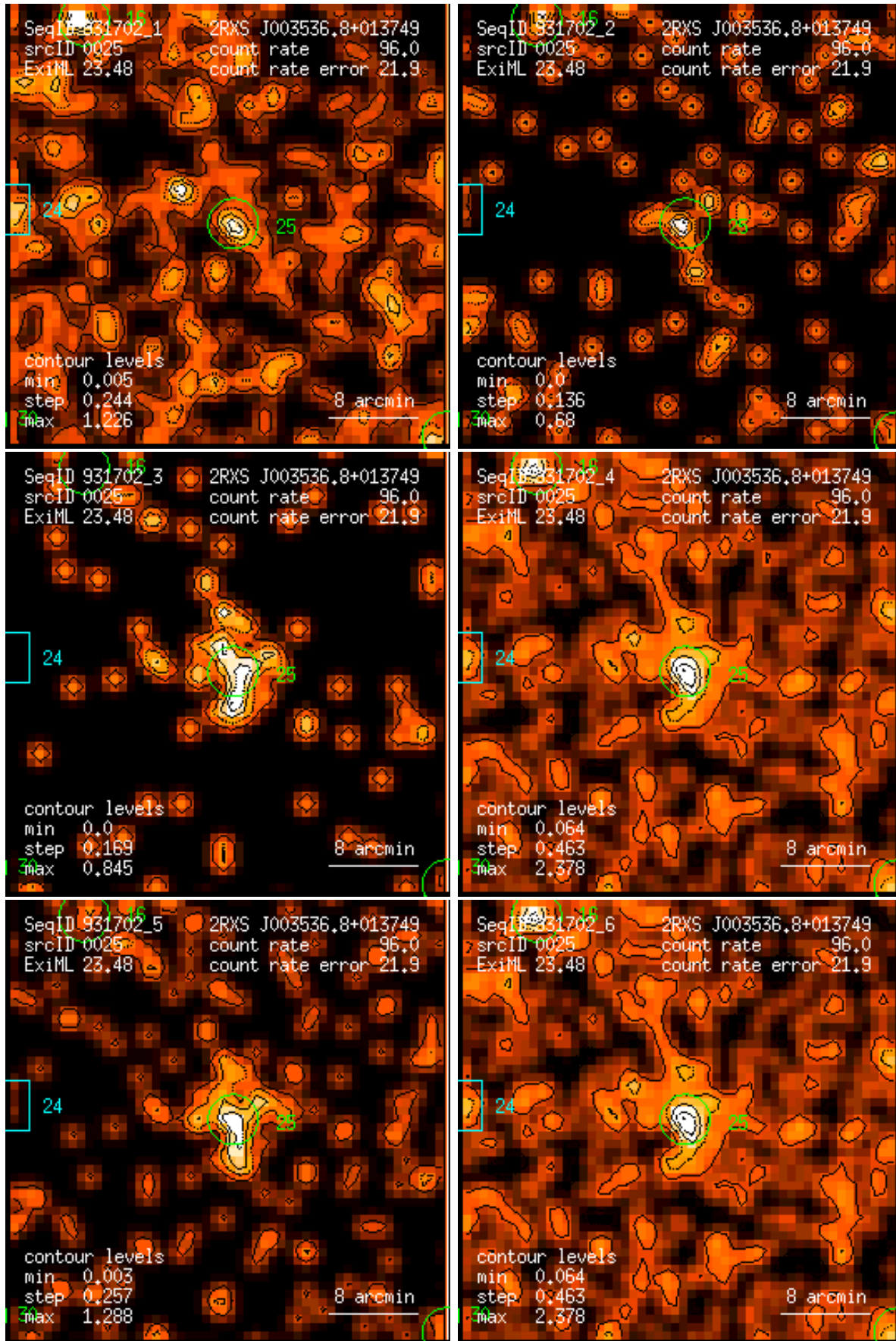
Figure 25: RASS 931702: detection 0025: band rate images, Gaussian filter: (1) PSPC channels 11 – 41, (2) 52 – 90, (3) 91 – 201, (4) 11 – 235, (5) 52 – 201, (6) 11 – 201. Broad band rates in counts/ks. Band rate contour levels in counts/ks/arcmin 2 .
