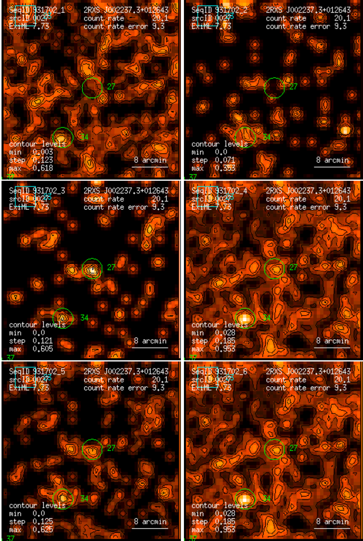
Figure 27: RASS 931702: detection 0027: band rate images, Gaussian filter: (1) PSPC channels 11 – 41, (2) 52 – 90, (3) 91 – 201, (4) 11 – 235, (5) 52 – 201, (6) 11 – 201. Broad band rates in counts/ks. Band rate contour levels in counts/ks/arcmin 2 .
