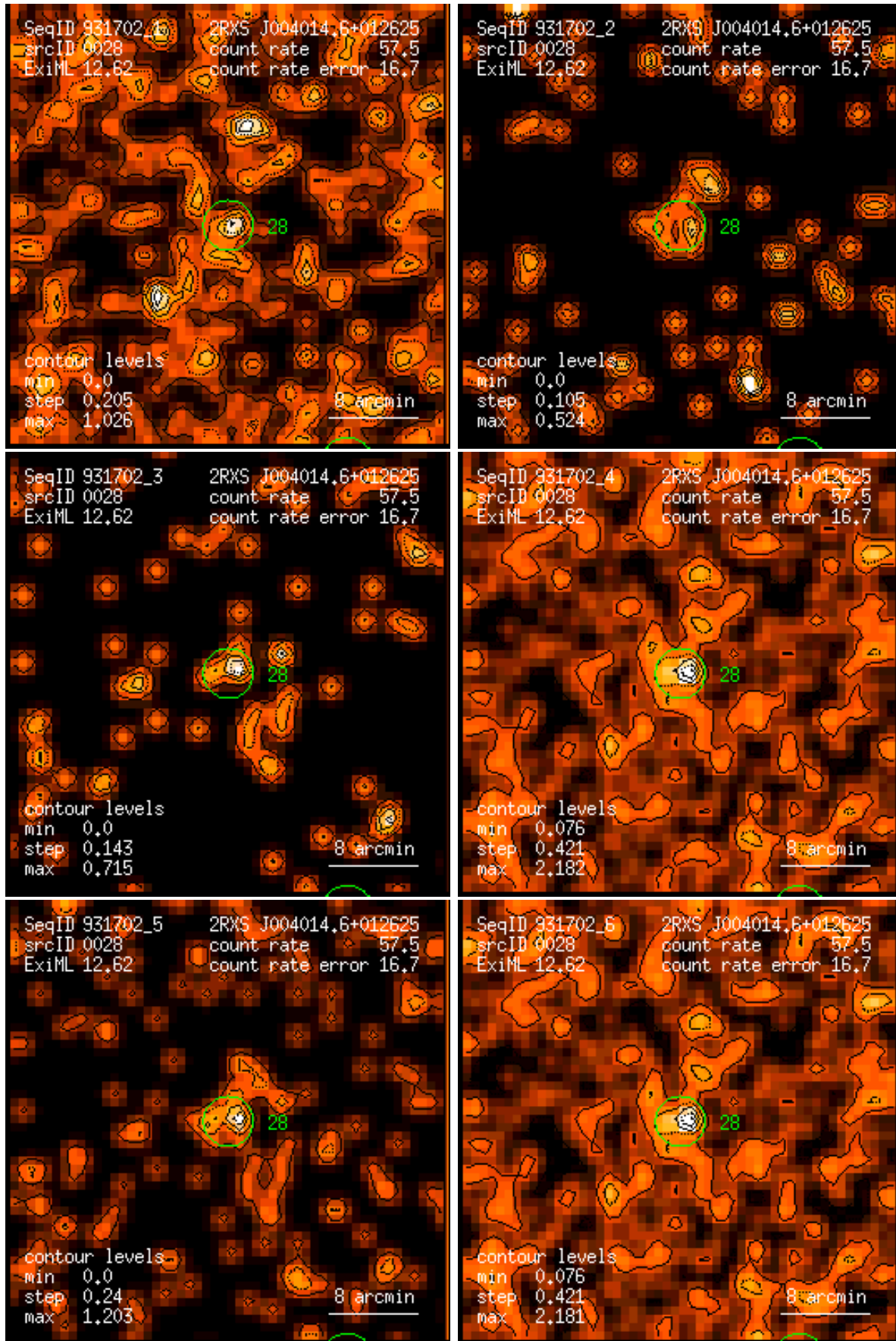
Figure 28: RASS 931702: detection 0028: band rate images, Gaussian filter: (1) PSPC channels 11 – 41, (2) 52 – 90, (3) 91 – 201, (4) 11 – 235, (5) 52 – 201, (6) 11 – 201. Broad band rates in counts/ks. Band rate contour levels in counts/ks/arcmin 2 .
