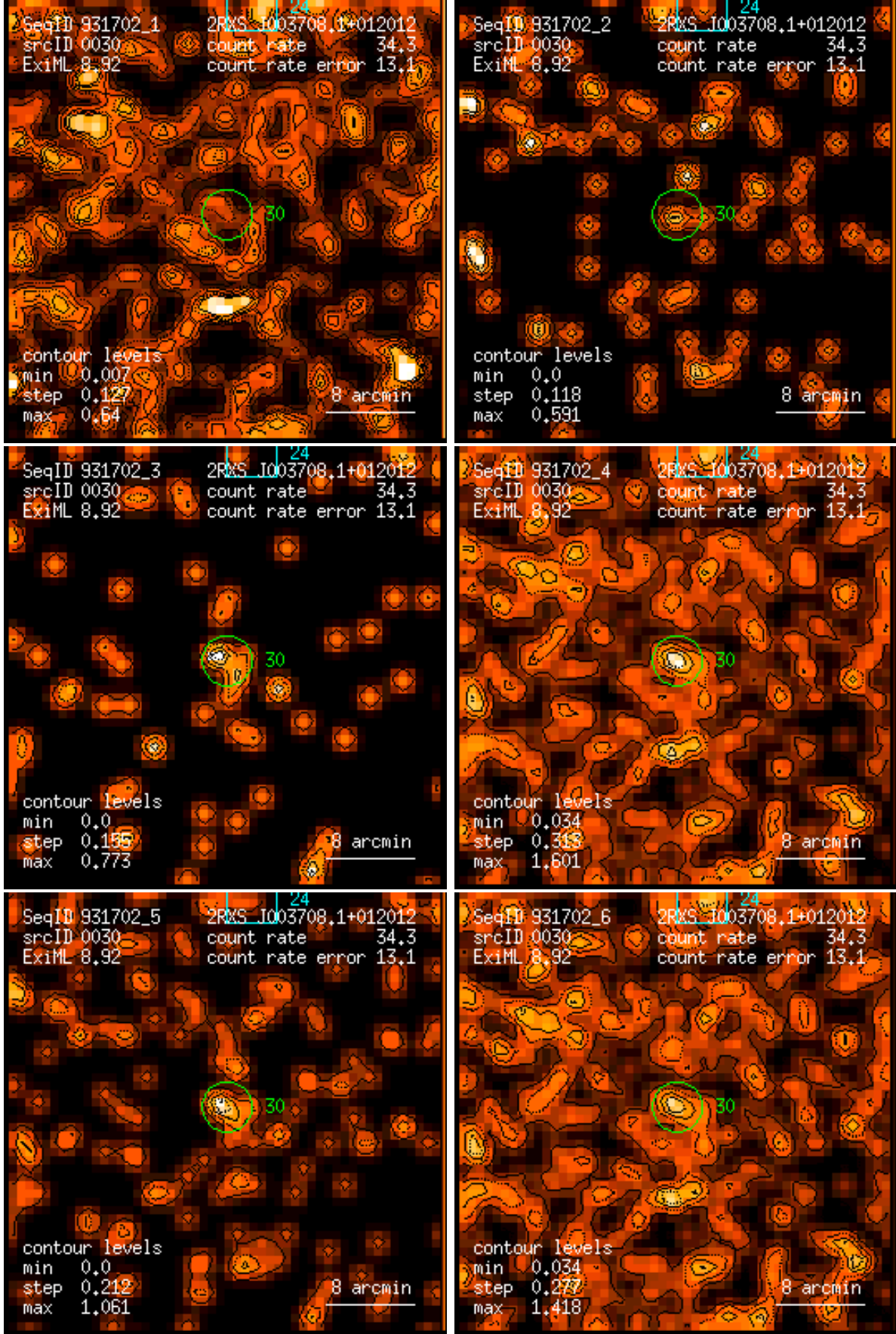
Figure 30: RASS 931702: detection 0030: band rate images, Gaussian filter: (1) PSPC channels 11 – 41, (2) 52 – 90, (3) 91 – 201, (4) 11 – 235, (5) 52 – 201, (6) 11 – 201. Broad band rates in counts/ks. Band rate contour levels in counts/ks/arcmin 2 .
