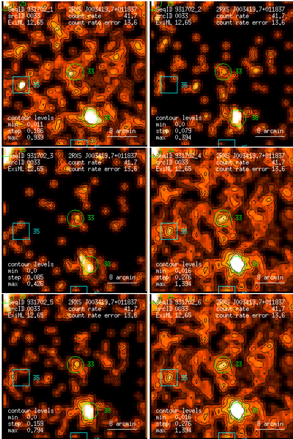
Figure 33: RASS 931702: detection 0033: band rate images, Gaussian filter: (1) PSPC channels 11 – 41, (2) 52 – 90, (3) 91 – 201, (4) 11 – 235, (5) 52 – 201, (6) 11 – 201. Broad band rates in counts/ks. Band rate contour levels in counts/ks/arcmin 2 .
