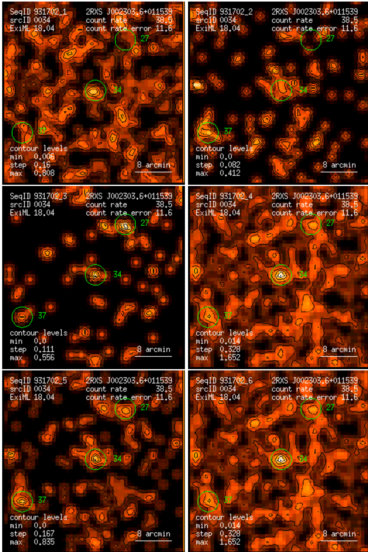
Figure 34: RASS 931702: detection 0034: band rate images, Gaussian filter: (1) PSPC channels 11 – 41, (2) 52 – 90, (3) 91 – 201, (4) 11 – 235, (5) 52 – 201, (6) 11 – 201. Broad band rates in counts/ks. Band rate contour levels in counts/ks/arcmin 2 .
